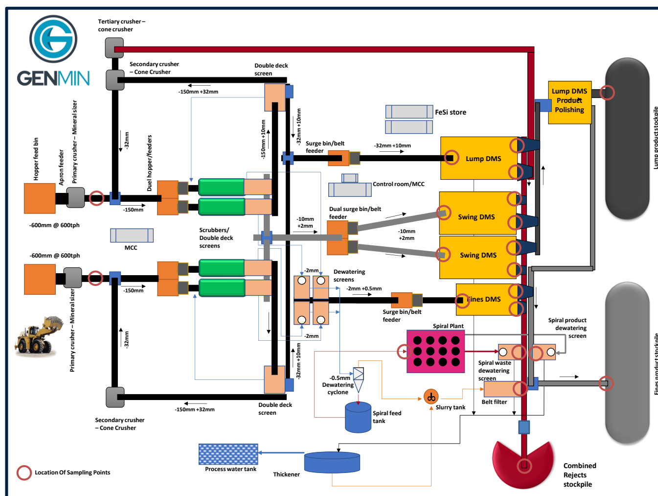
Figure 11: Block flow diagram of the proposed flowsheet
