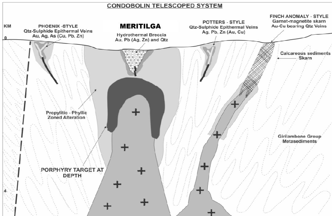
Schematic model for mineralisation in the Condoobolin Mineral Field.
