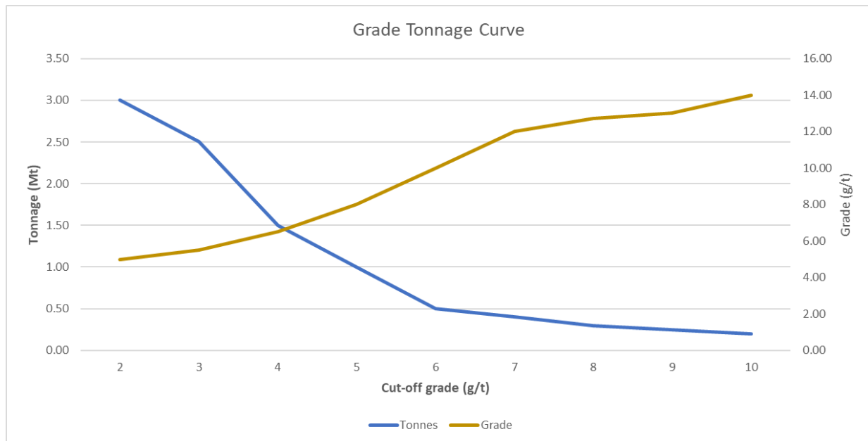
Figure 8 – Grade-tonnage curve for the Labyrinth Inferred Mineral Resource.
