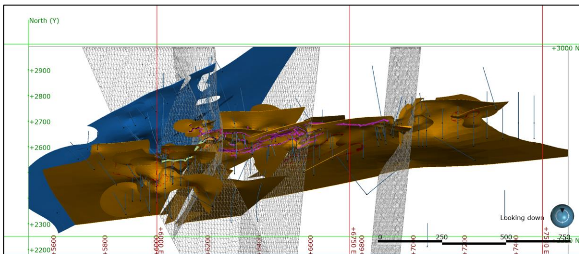
Figure 4 – Plan view of the Main-lode (orange) and Boucher (blue) estimation domains.
