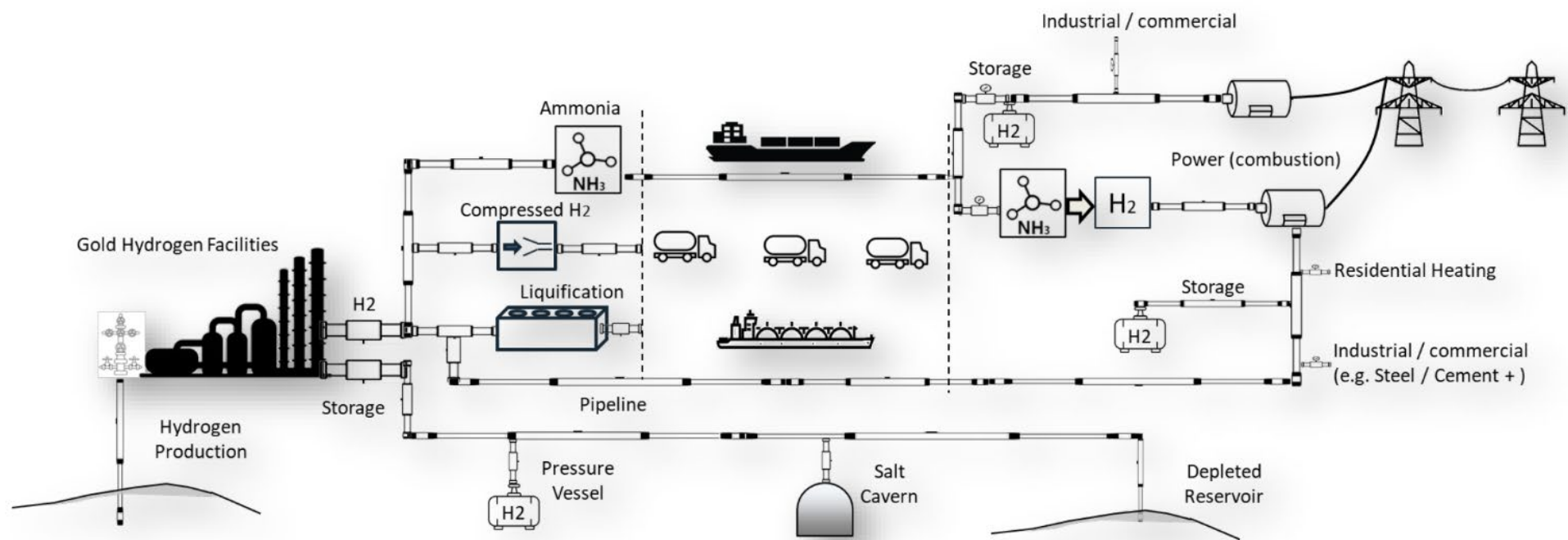
Examples of Downstream Hydrogen Distribution and Usage
