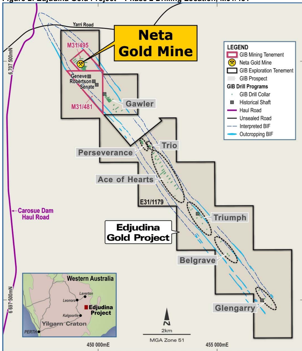
Figure 2: Edjudina Gold Project – Phase 2 Drilling Location, M31/481
