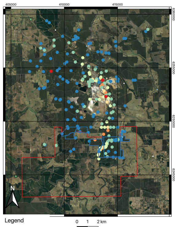
Figure 5: Sn anomaly
