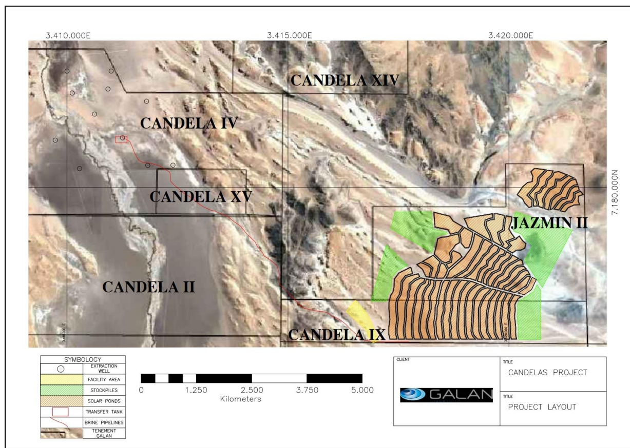
Figure 7: Candelas Ponds Layout
