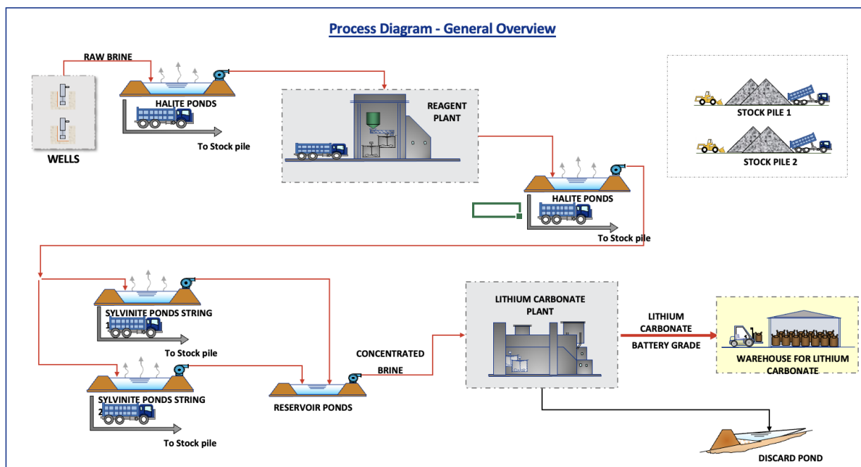
Figure 6: Process Flow Diagram Candelas Project
