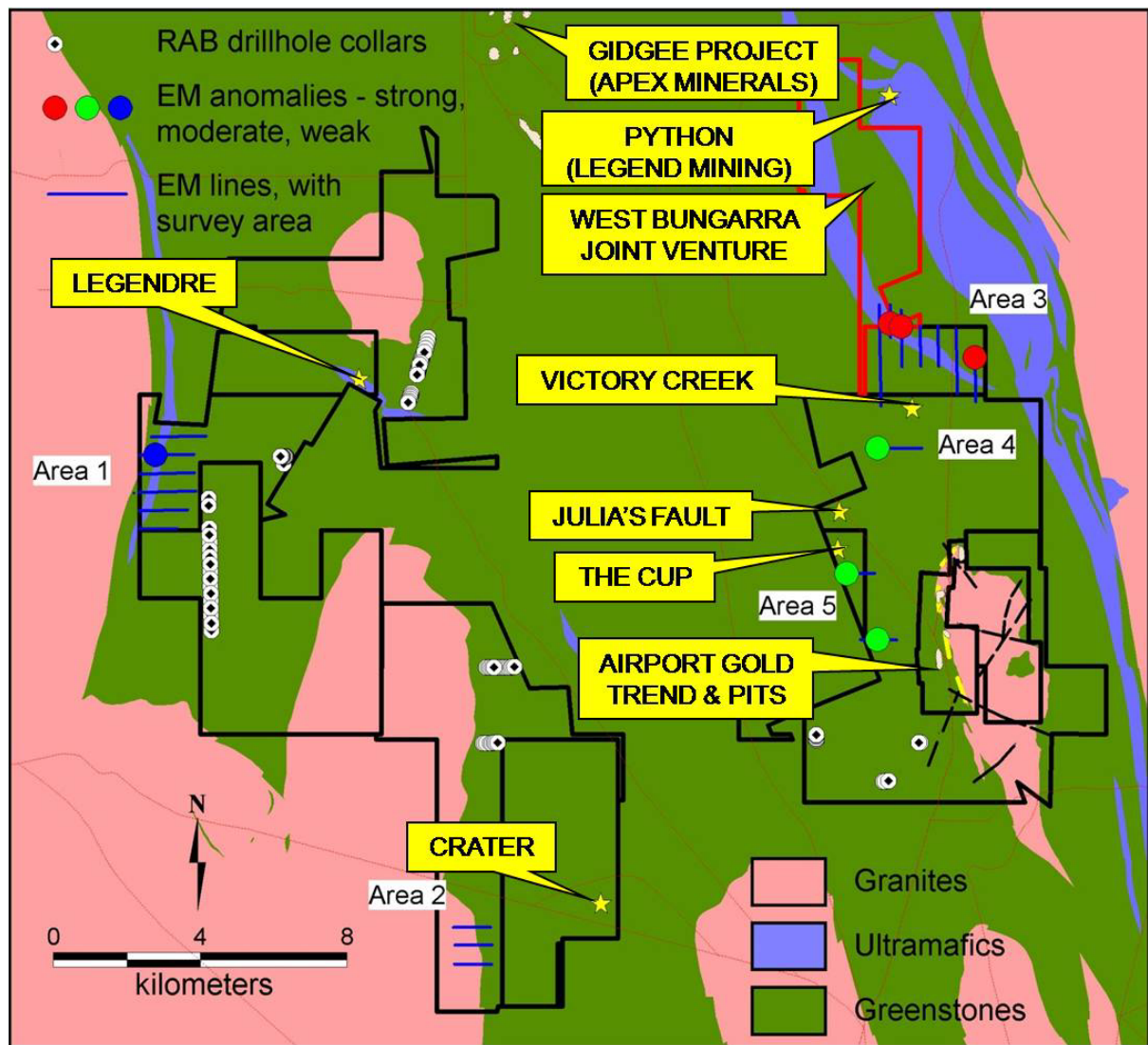
Figure 2. Prospect locations and location of current RAB drillholes and EM survey lines, Gidgee Project
