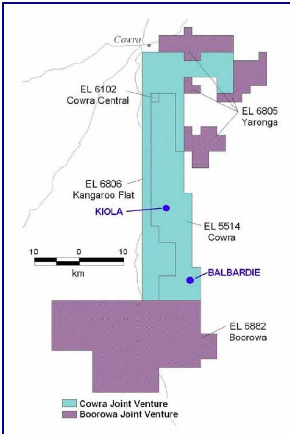
Figure 3. Cowra JV area, showing prospect locations. Gateway's interest is within the "Cowra Joint Venture" only. (From Minotaur release, 27/11/2008)
