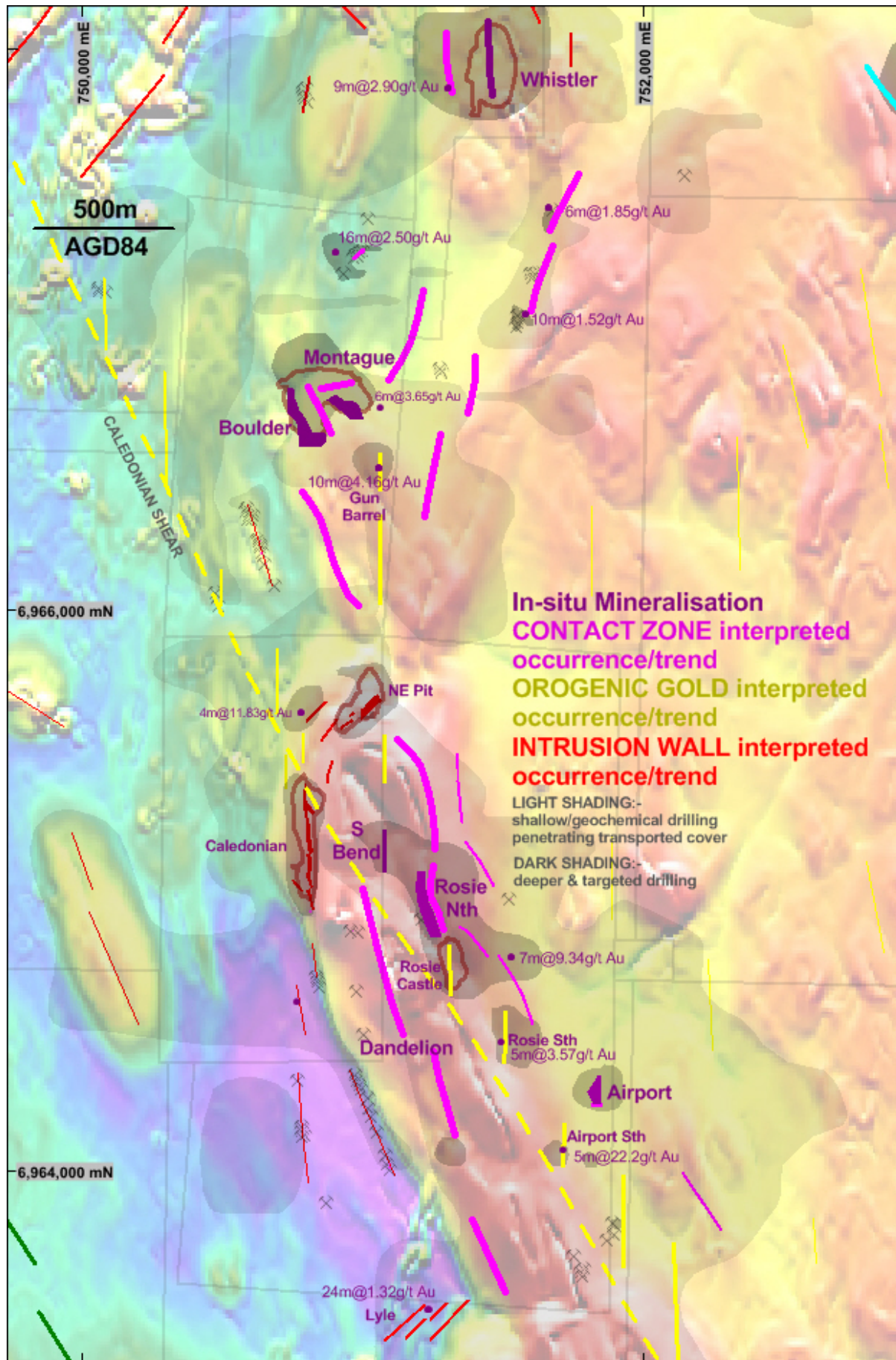
Magnetic Survey and mineralising zones of the Montague System and proximal Intrusion Wall
