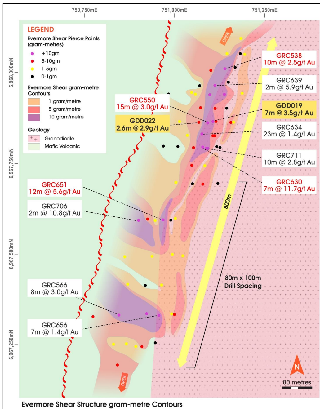
Figure (3): Evermore Shear interpretation gram-metre contour plan with associated pierce points. Note open ends along strike and extensive zone of wide-spaced drill coverage
