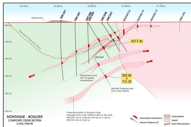
Figure (4): Montague-Boulder composite cross section highlighting potential repeat shears beneath the current Mineral Resource interpretation and AUD$2,400/oz constraining shell
