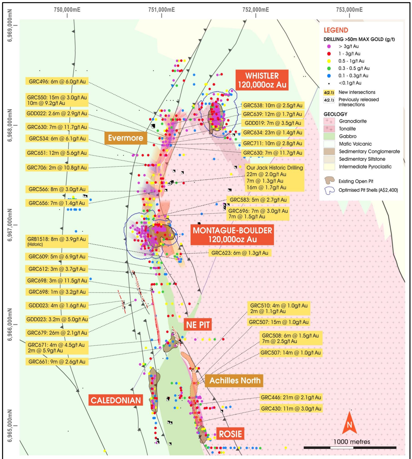
Figure (2): Northwest Margin compiled interpretation detailed plan(including significant intercepts) with strategic prospects for Resource upgrade. Note the interpreted new high-grade zones at Evermore, Achilles North and immediately east of the Montague-Boulder pit.
