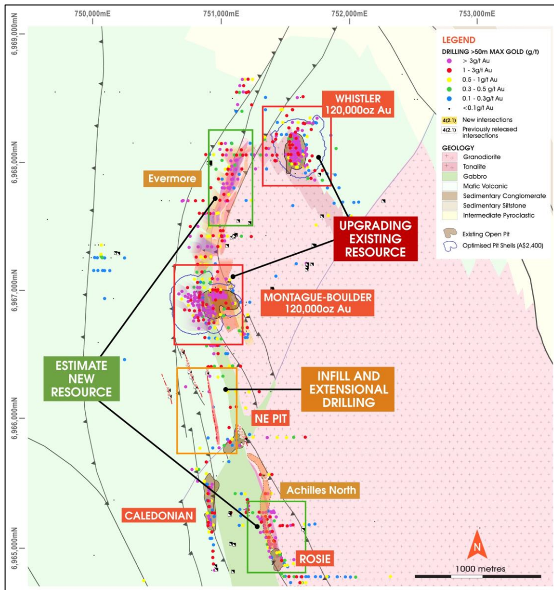
Figure (1): Northwest Margin compiled interpretation simplified plan with strategic prospects for Resource upgrade. Note the interpreted new high-grade zones at Evermore, Achilles North and immediately east of the Montague-Boulder pit.
