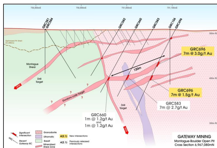
Figure (5): Montague-Boulder drill cross-section 6,967,080mN. Note the proximity of this new structure to the existing Mineral Resource interpretation and AUD$2,400/oz constraining shell
