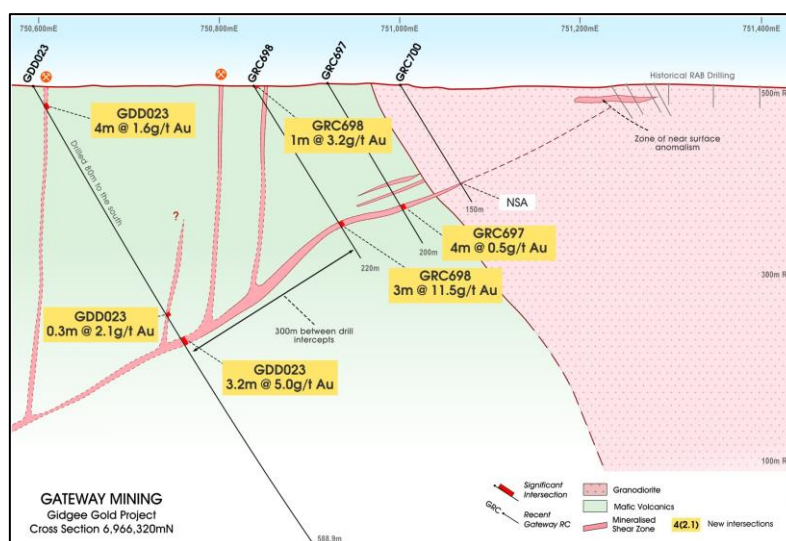
Figure (6): Montague-Boulder to Northeast Pit drill cross-section 6,966,320mN. Note hole GDD023 has been projected from 80m south.
