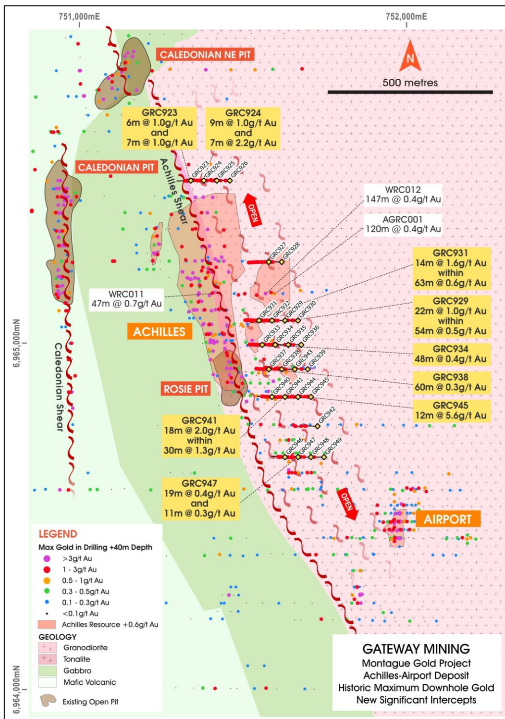
Figure (2): Achilles Deposit with existing Mineral Resource outline, and location of new intersections. Note the extensions of shallow mineralisation immediately along strike to the north, as well as broad scale moderate grade mineralisation hosted in granodiorite east of the main mineralised Achilles structure.
