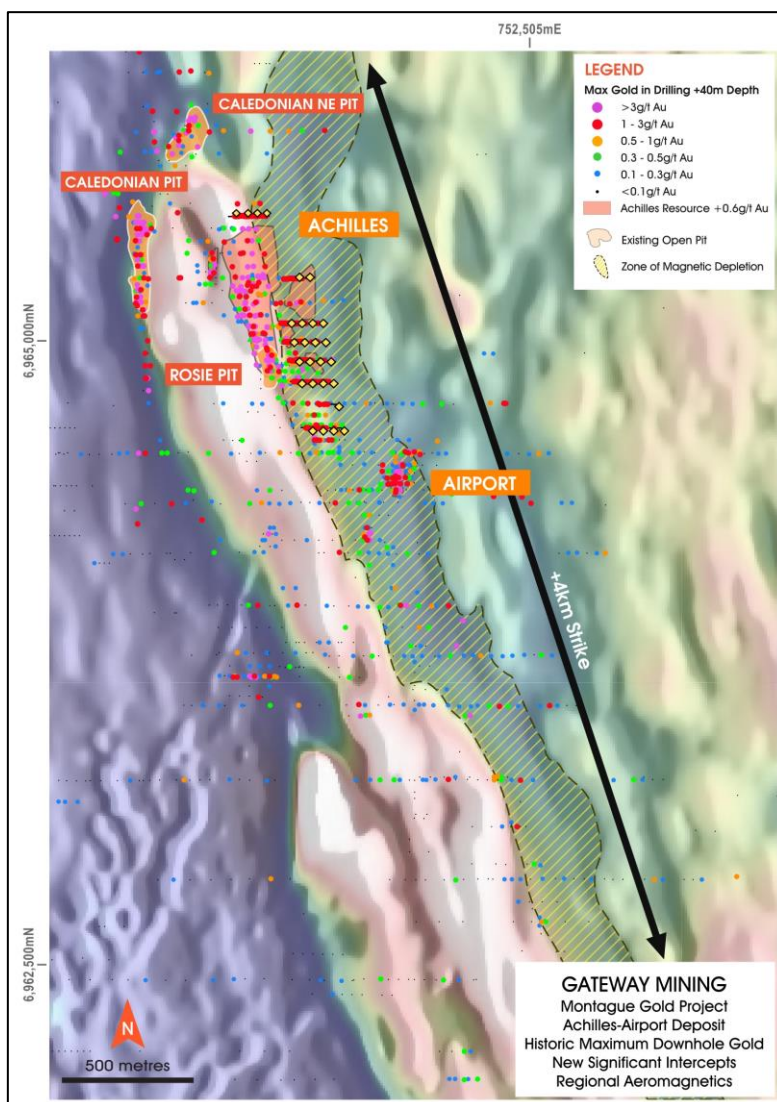
Figure (4): Broader Achilles deposit and large scale target within the Montague Granodiorite, highlighted by the zone of magnetic depletion in the Montague Granodiorite.
