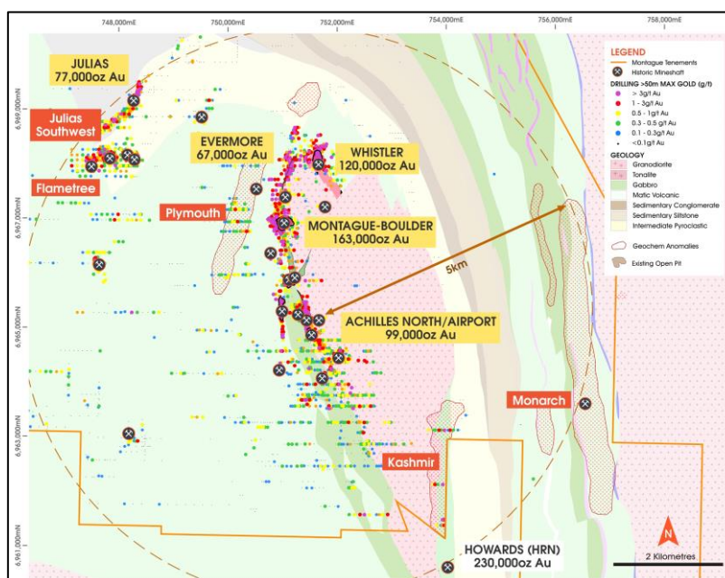
Figure (1): Achilles deposit location, showing existing Mineral Resources within the Montague Gold Project.
