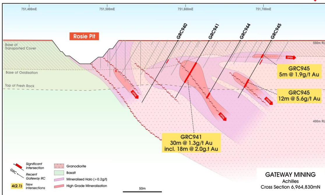
Figure (3): Achilles East cross-section 6,964,830mN with the broad scale mineralisation in the Montague Granodiorite relative to the shear hosted mineralisation targeted in the historic Rosie open pit.
