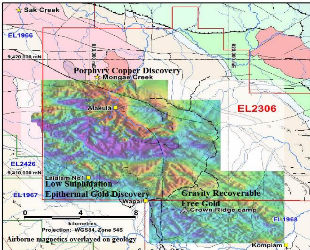
Figure 6: Expanded exploration program to aggressively investigate other potential mineral systems including at Laialam and Mongae Creek
