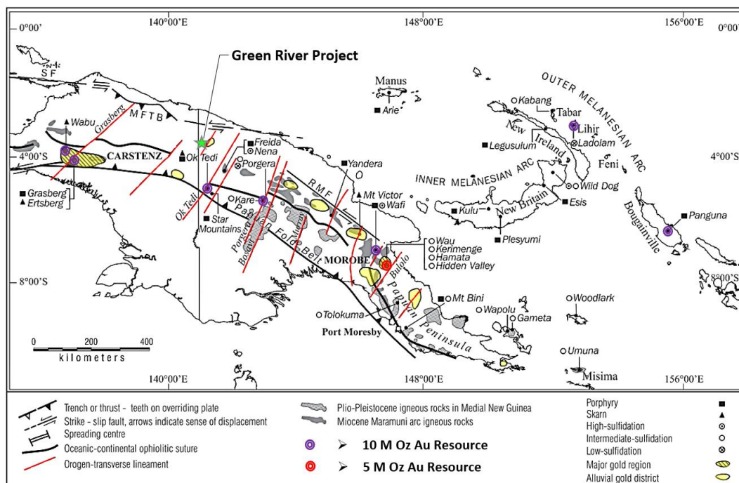
Figure 1. Location of the Green River Project in relation to alluvial goldfields, transverse structures and the known extent of the Maramuni Suite. Modified from Garwin et al (2005).
