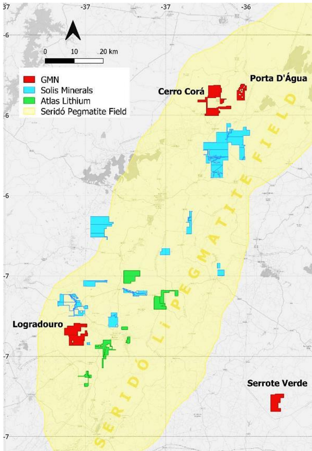
Figure 11. Location of the Cerro Corá-Porta D'água, Logradouro and Serrote Verde tenements in relation to the Seridó Li-Pegmatite field and major lithium explorers.
