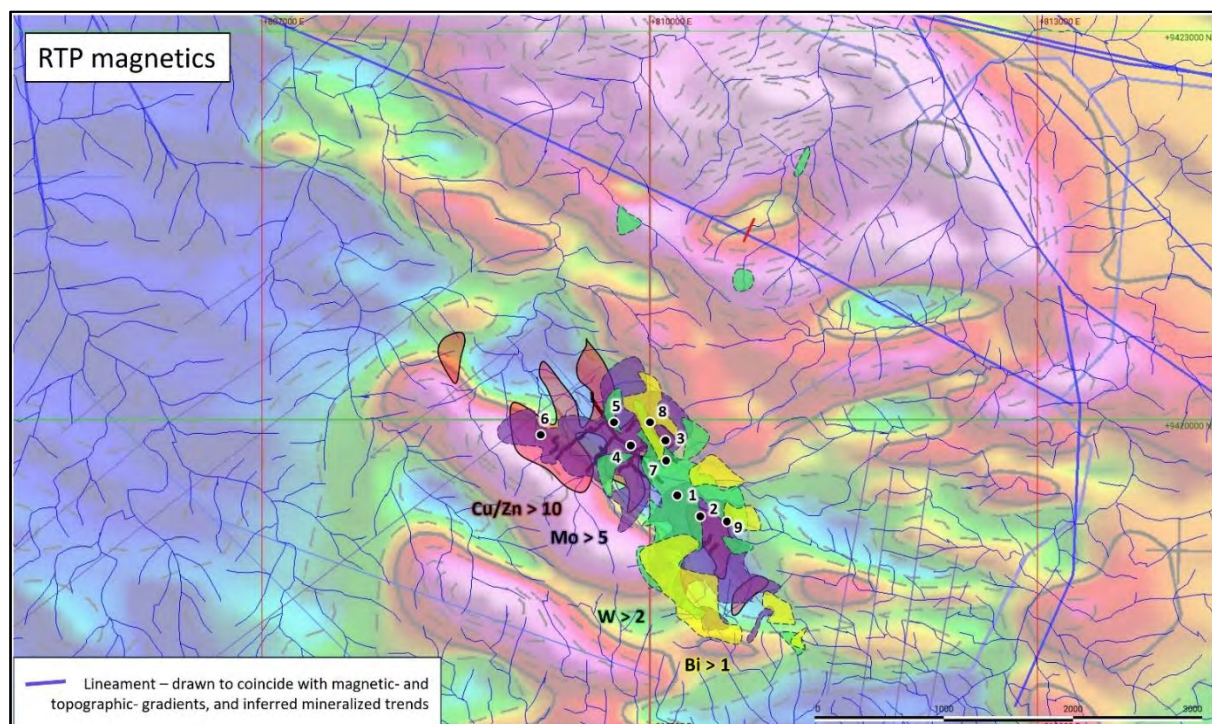
Figure 12: RTP magnetics data showing interpreted structural trends in relation Cu/Zn, Mo, W and Bi anomalies from soil auger sampling at Monoyal-Mongae Creek.
