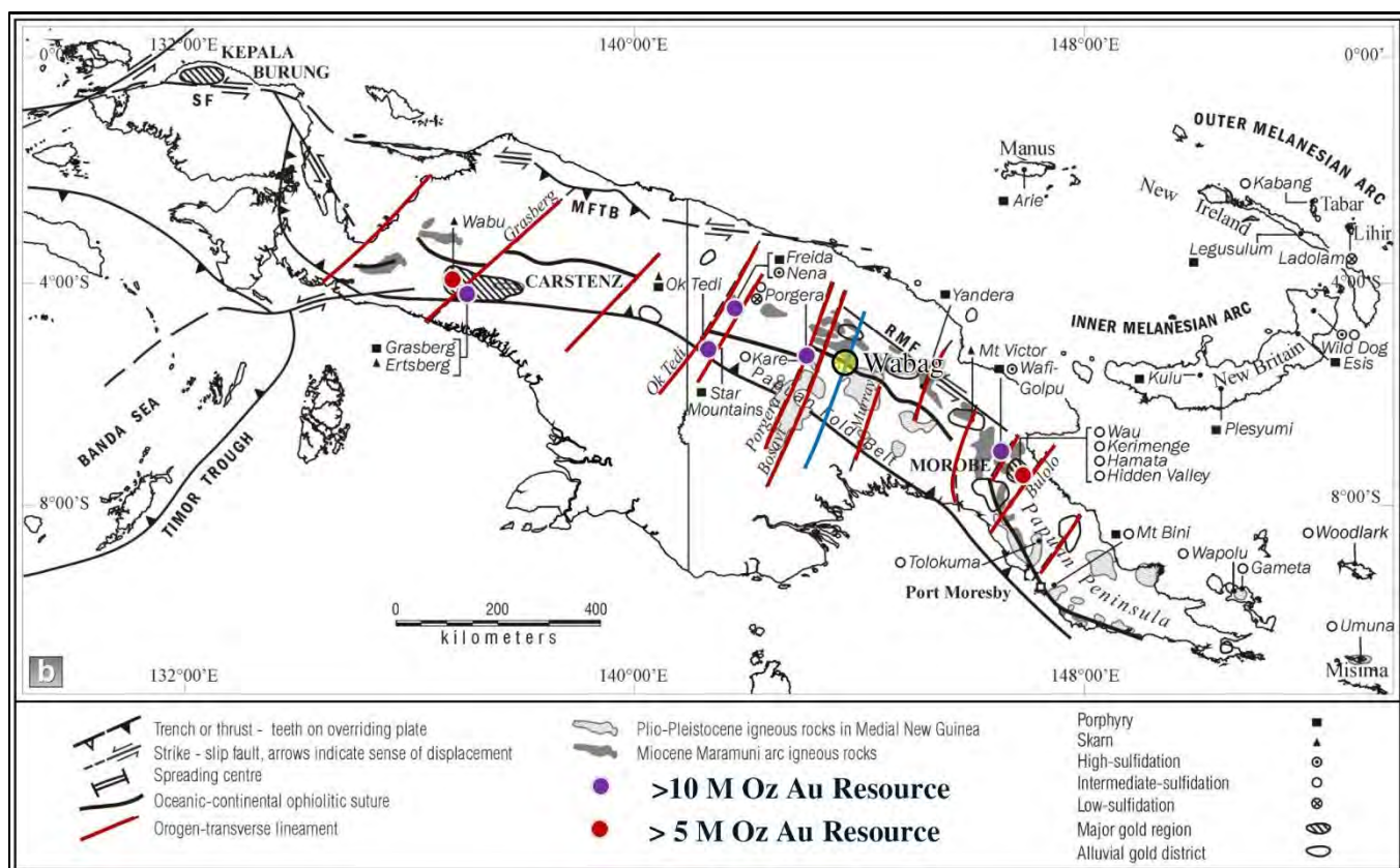
Figure 2: Regional Geological and mineralization setting of Papua New Guinea.
