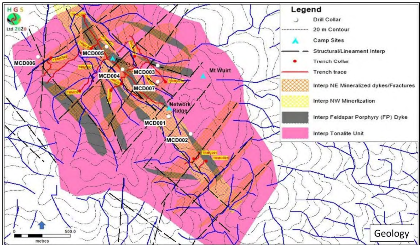
Figure 11: Local geological setting at Mongae Creek.
