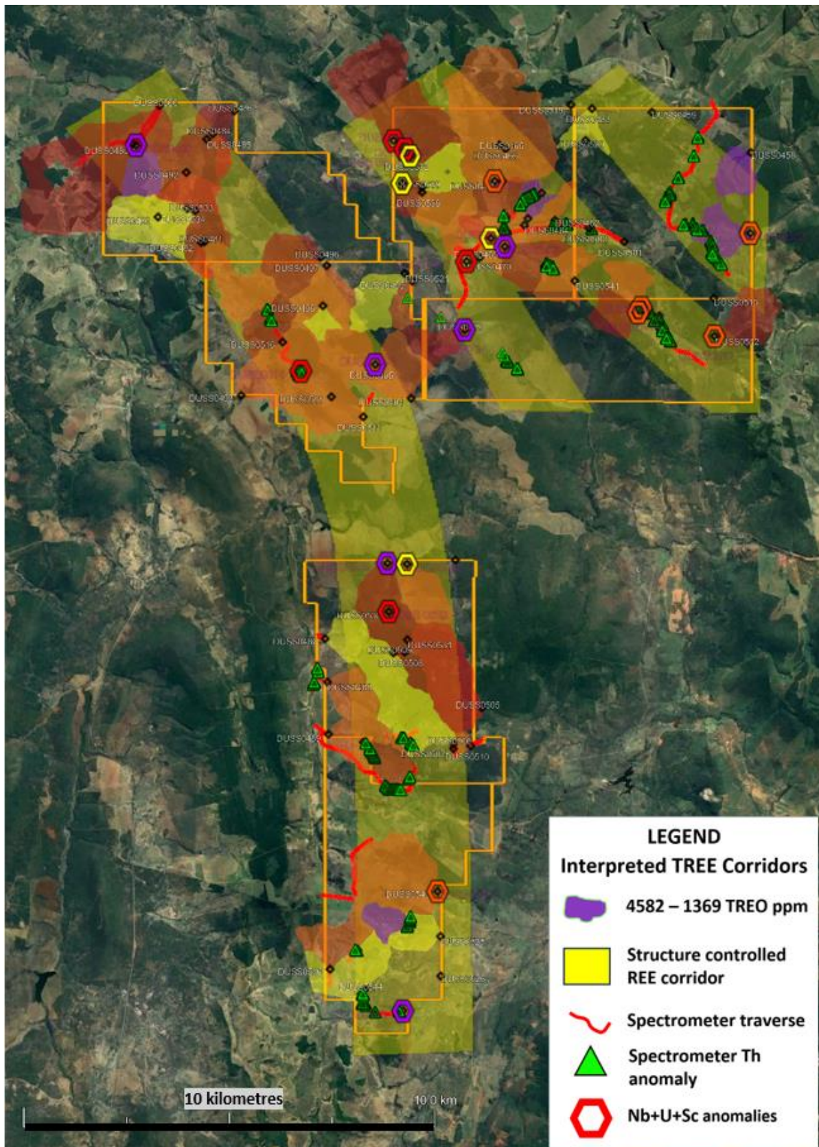
Figure 3. Interpreted Structural or stratigraphic controls on mineralised catchments. Yellow corridors follow regional structure, parallel to a fold seen as vegetated inverted U shapes immediately west of the southern tenements. A dome to the east controls part of the two northeast structures.
