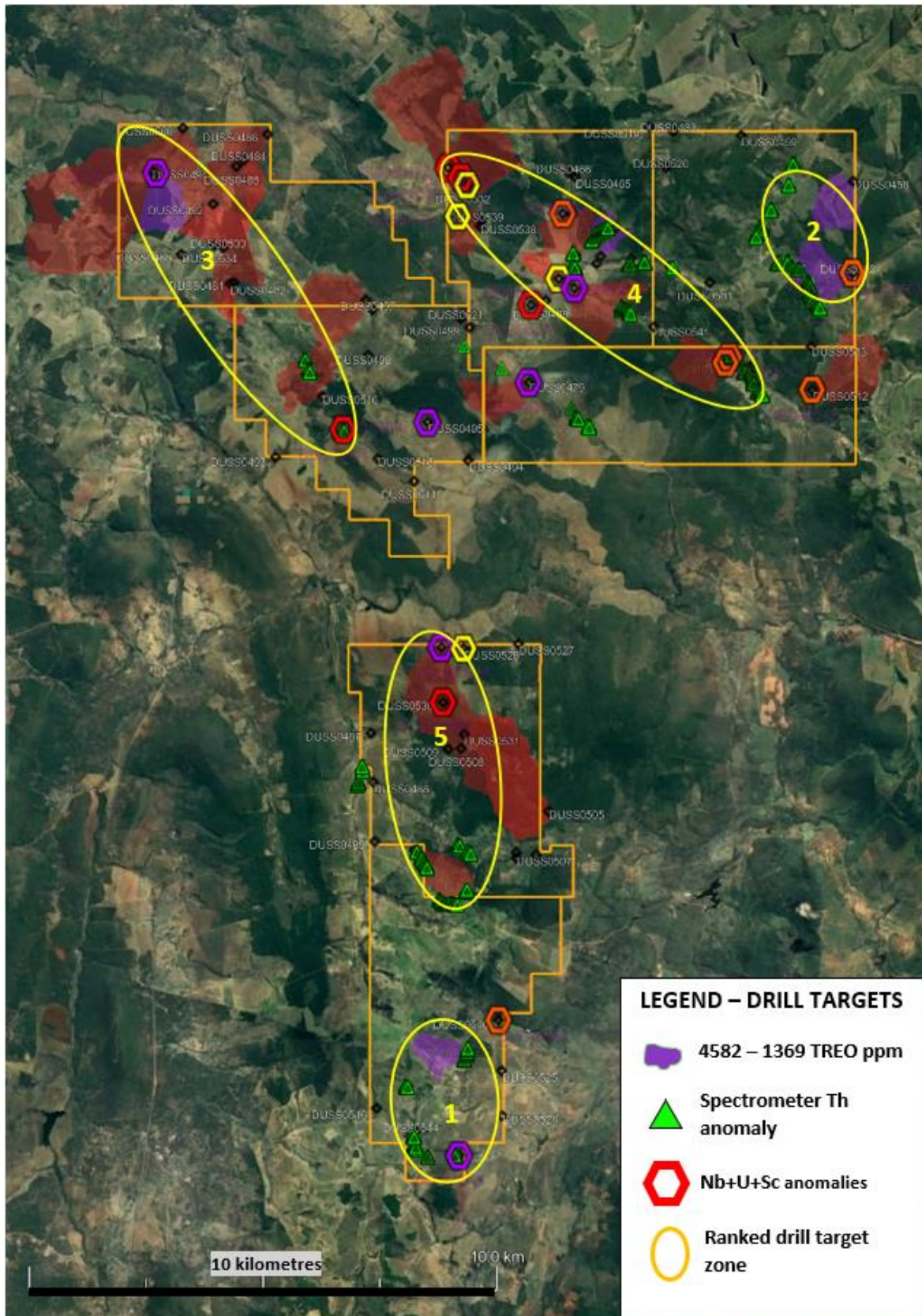
Figure 4. Ranked drilling target zones for first pass auger drilling followed up by diamond drilling of ultrahigh grade monazite mineralisation and Sonic or RC drilling of IAC resources. High grade stream sediment samples, coupled with the Nb-U-Sc anomalies is considered indicative of ultra-high grade hard rock mineralisation.
