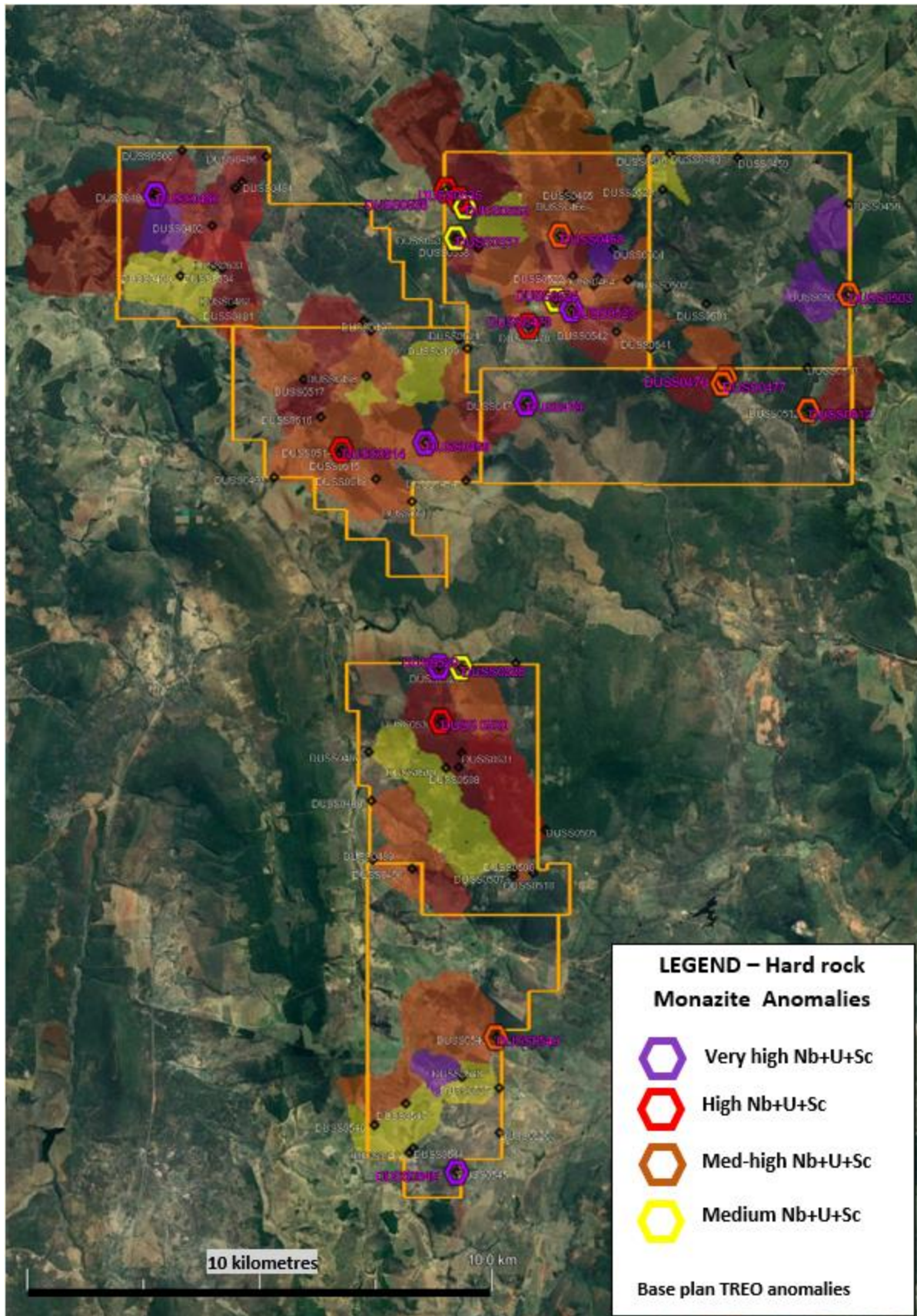
Figure 2. Combined niobium-uranium-scandium anomalies, indicative of hard rock monazite type mineralisation, a major focus of GMN exploration.
