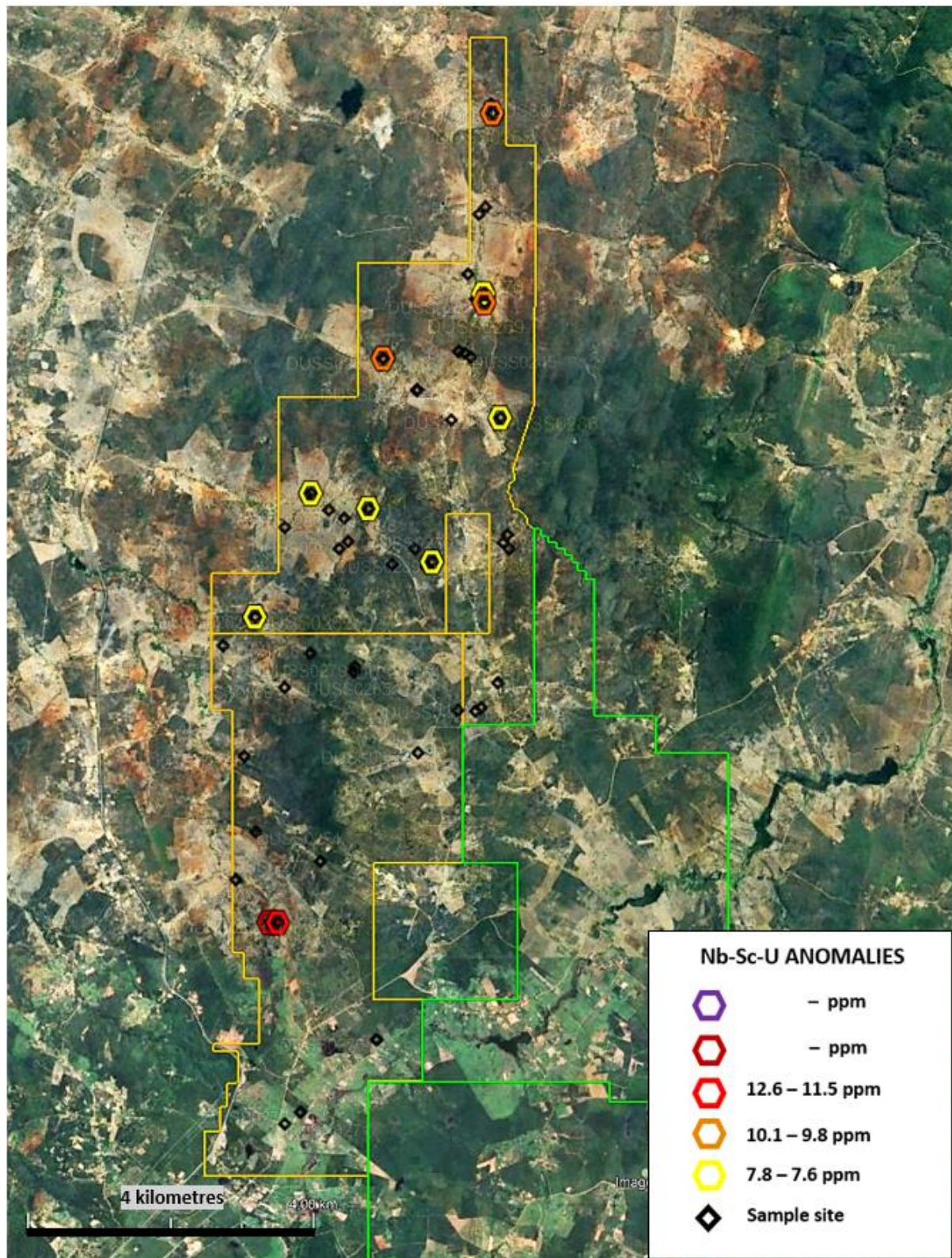
Figure 3. Stream sediment anomalies indicative of hard rock ultra-high grade type mineralisation.
