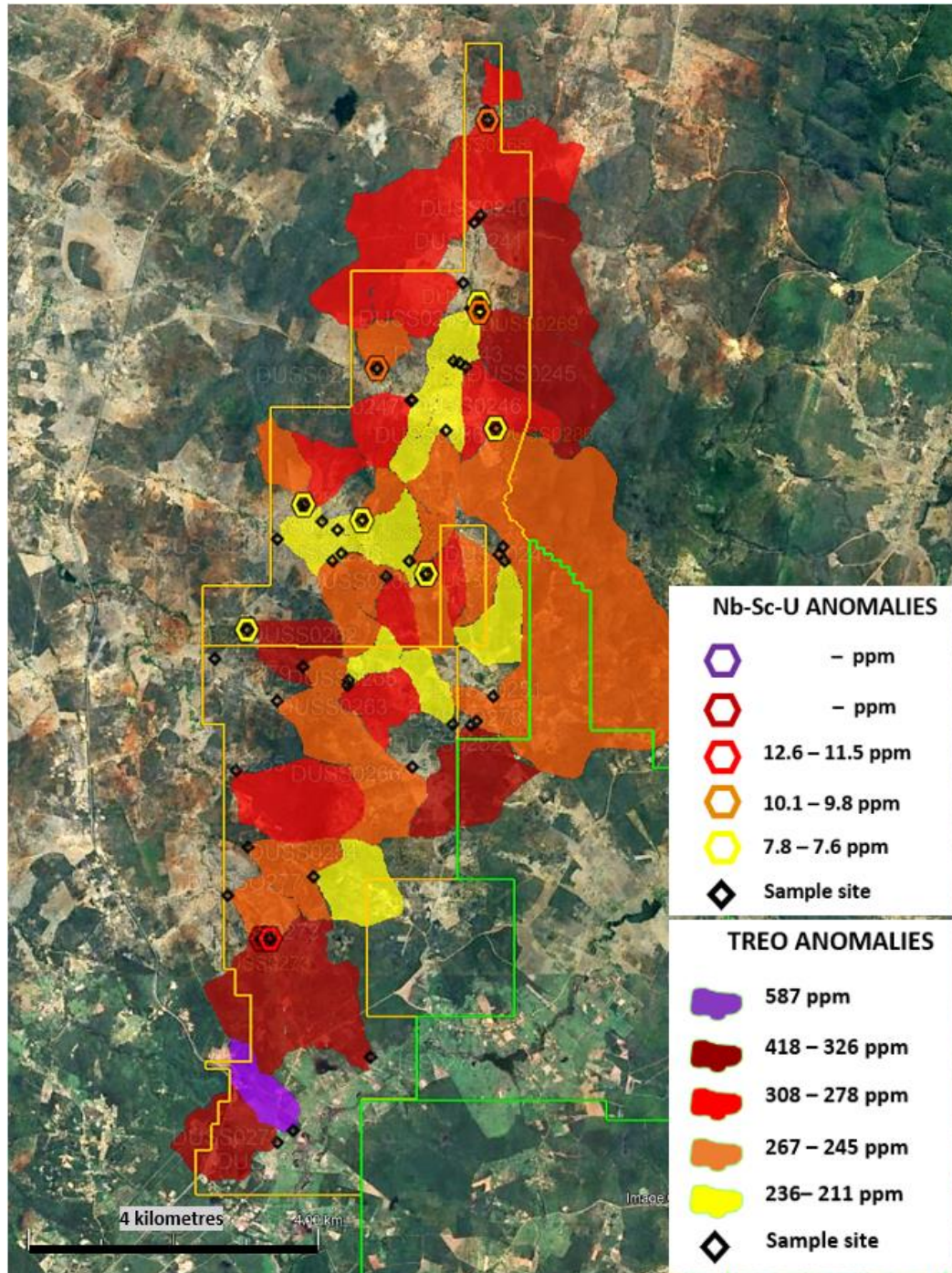
Figure 4. TREO anomalies plotted as anomalous stream sediment catchments. Maximum value of 587 ppm TREO. New data added additional very high TREO values in the highest (purple) category. High grade stream sediment samples, coupled with the Nb-U-Sc anomalies (hexagons - see figure 3 for legend) are considered indicative of ultra-high grade hard rock mineralisation.
