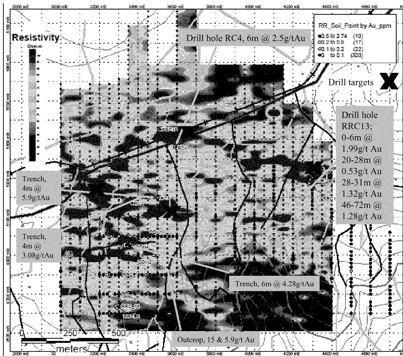
Figure 2. Raki Raki Project; Qalau-4300 Resistivity Gradient Array
