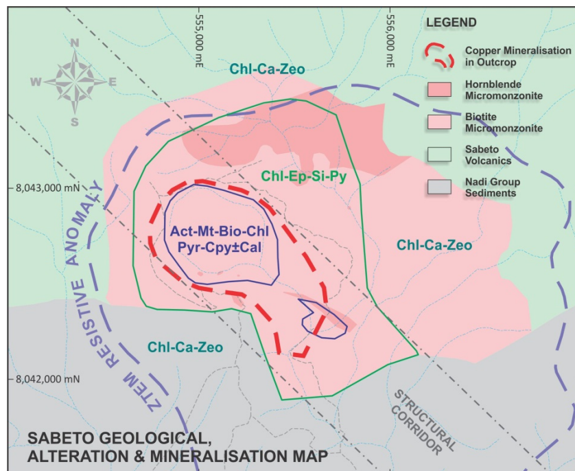
Figure 2: Geological map of Sabeto showing observed structure, alteration, mineralisation, and ZTEM anomaly.
