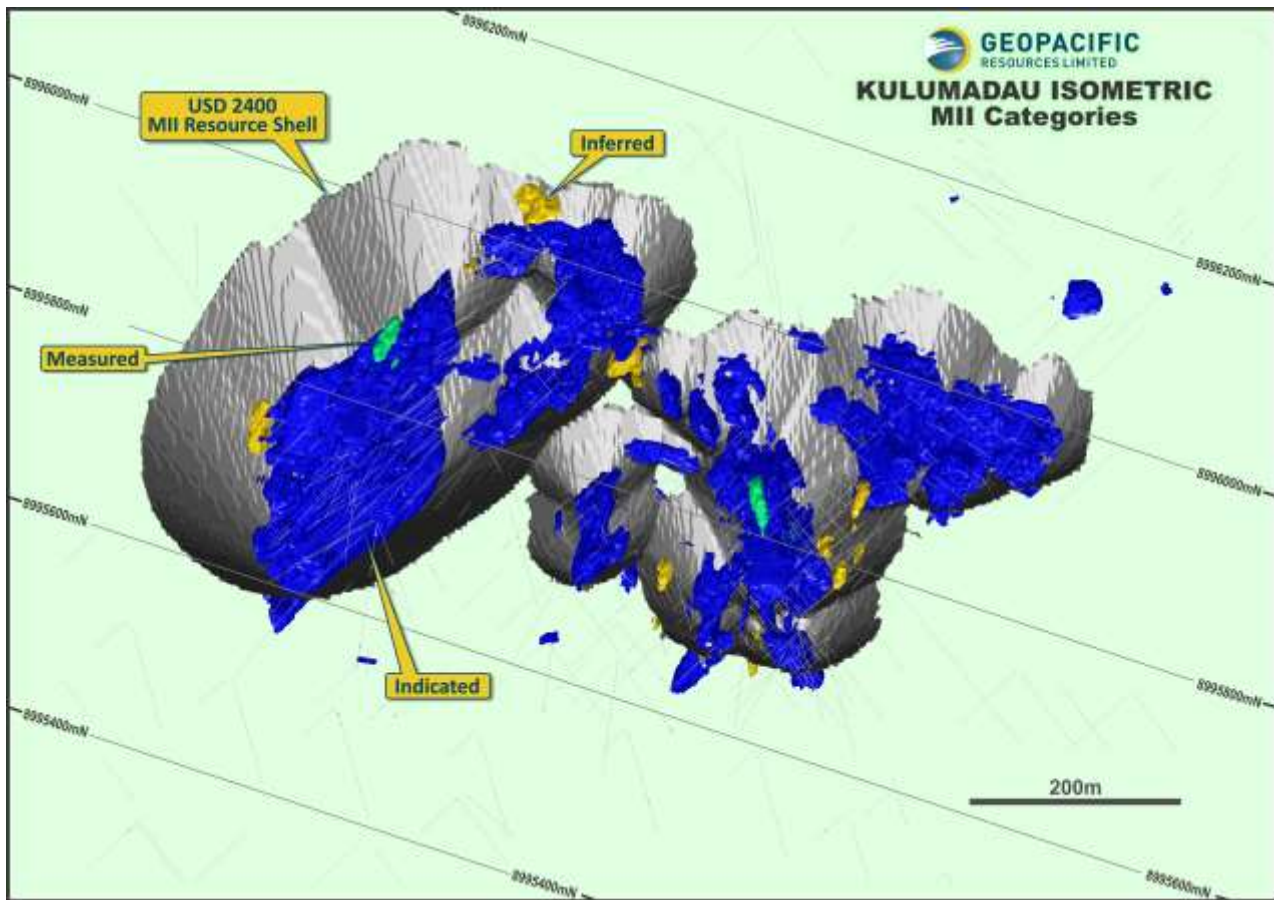
Figure 7 – Isometric view of Kulumadau showing resource classification
