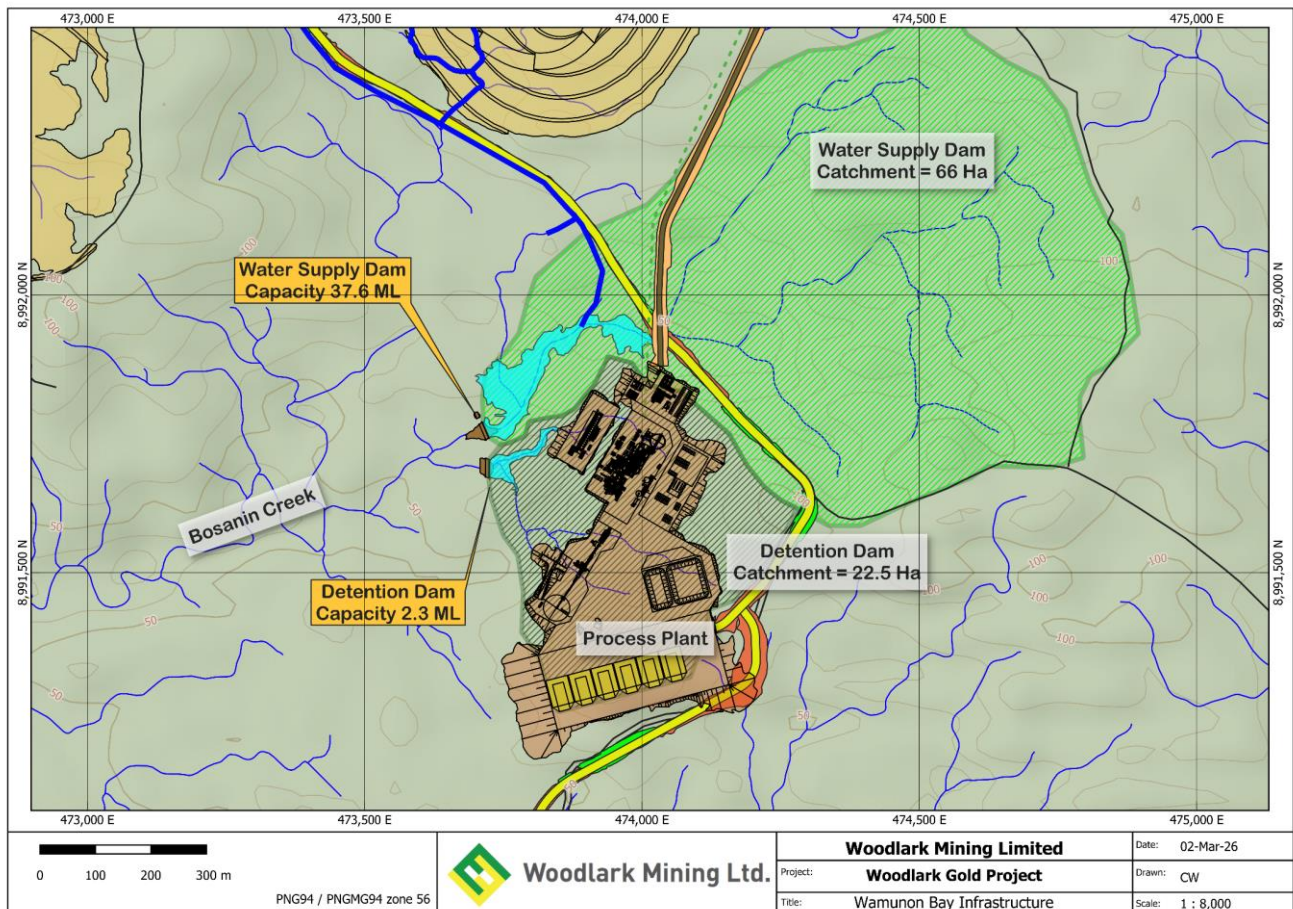
Figure 1.29 Water supply &amp; detention dams
