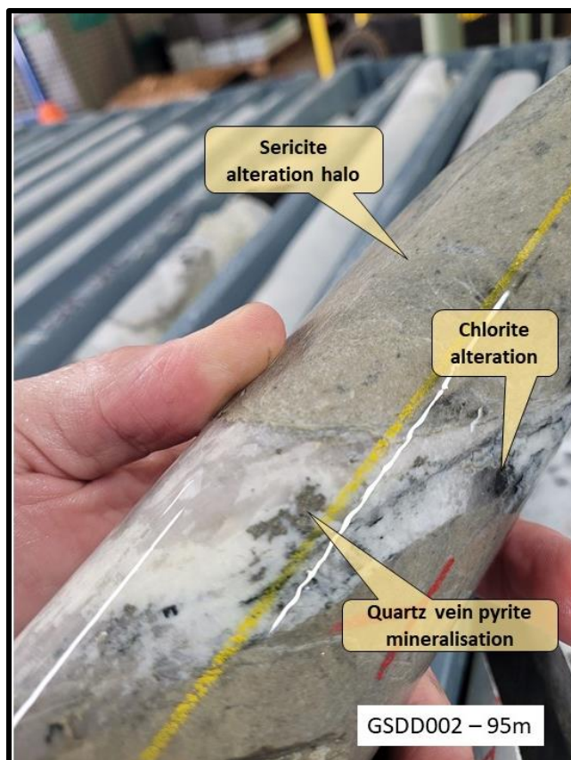
Image 4: Vein-hosted pyrite mineralisation with an intense sericite alteration halo from GSDD002 95m. The sericite is the light brown coloration in the core and is a common alteration mineral developed in gold mineralised systems.
