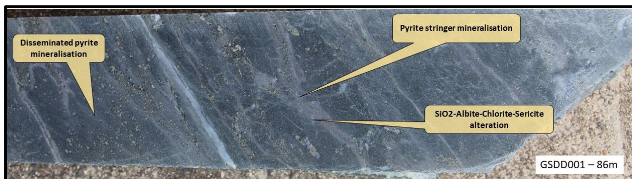
Image 1: Disseminated and stringer pyrite mineralisation in brecciated siltstone unit at 86m, GSDD001
