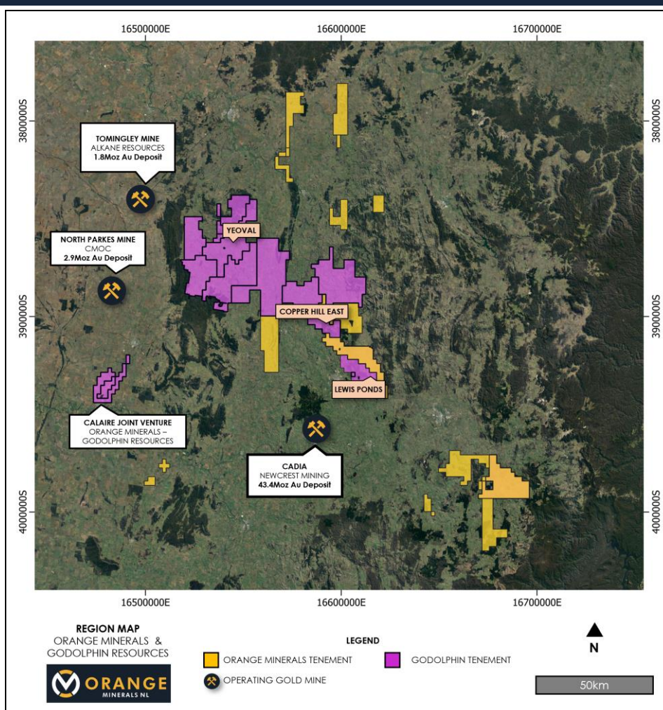
Figure 1 - Map of Orange Minerals NL and Godolphin Resources Ltd Projects in the Central Lachlan Fold Belt
