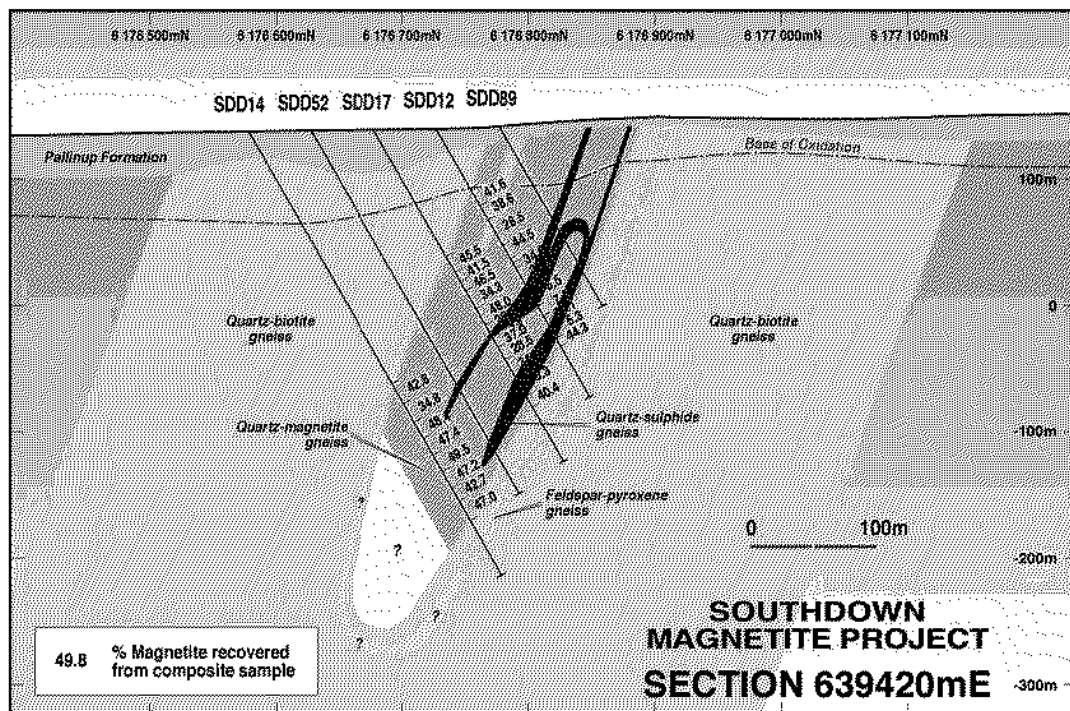
Figure 6: Interpreted Cross Section 639420mE
