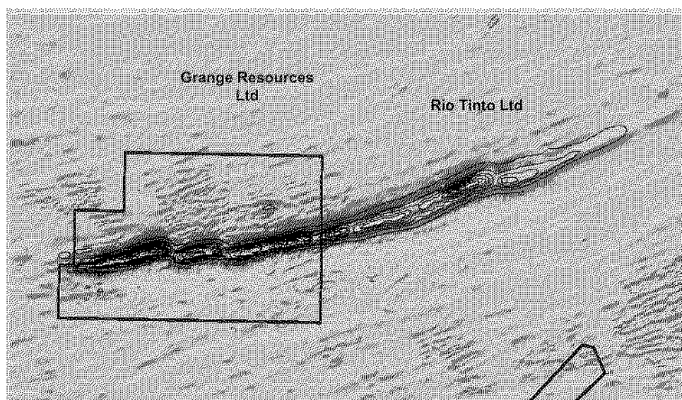
Figure 3: Rio Tinto Aeromagnetic Survey 2005
