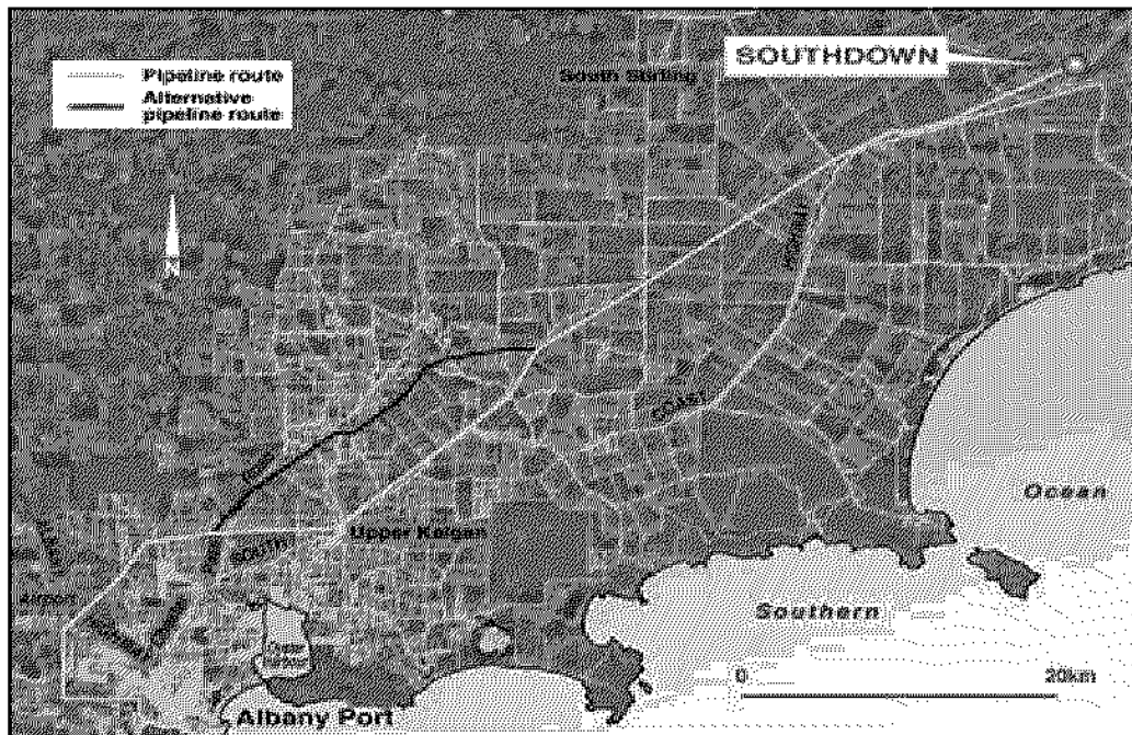
Figure 7: Proposed Slurry Pipeline Route
