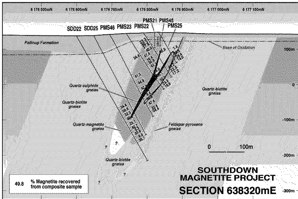
Figure 5: Interpreted Cross Section 638320mE
