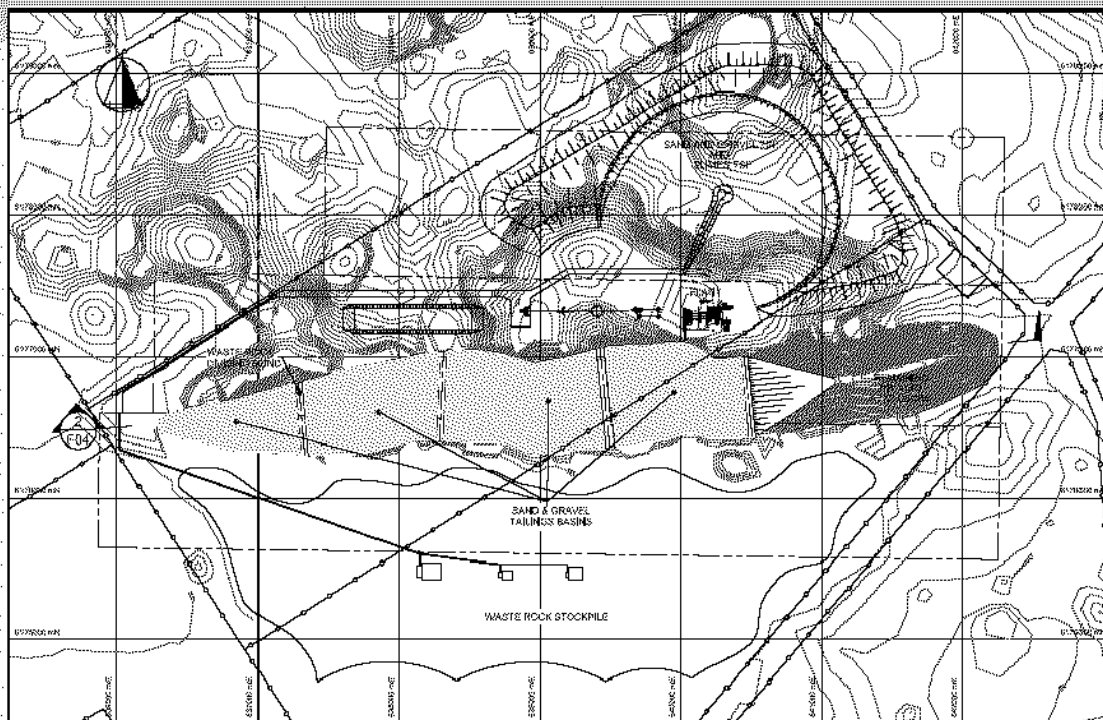
Figure 9: Conceptual site layout plan of surface and in-pit tailings storage facilities
