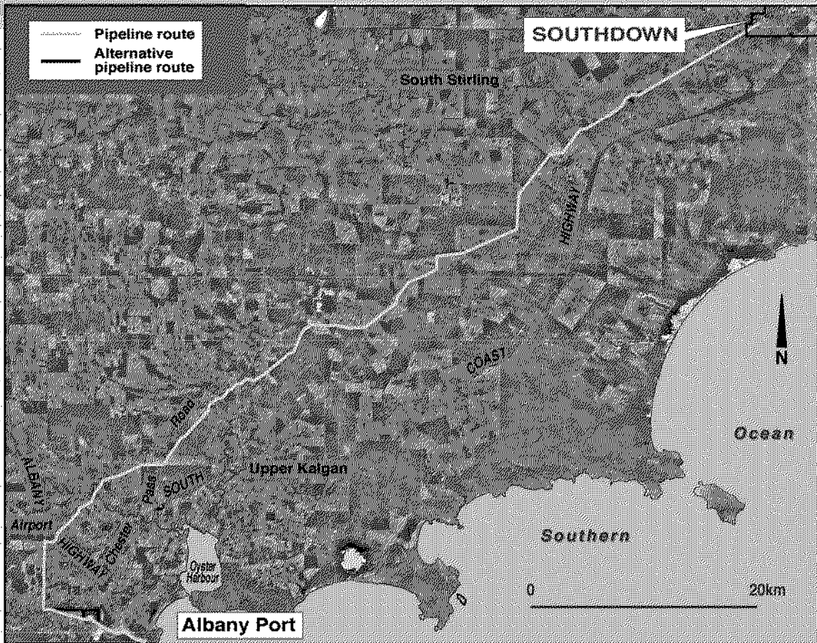
Figure 10: Proposed Slurry Pipeline Route
