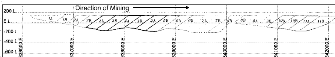
Figure 8: Conceptual open pit - long section looking north showing possible strip layout
