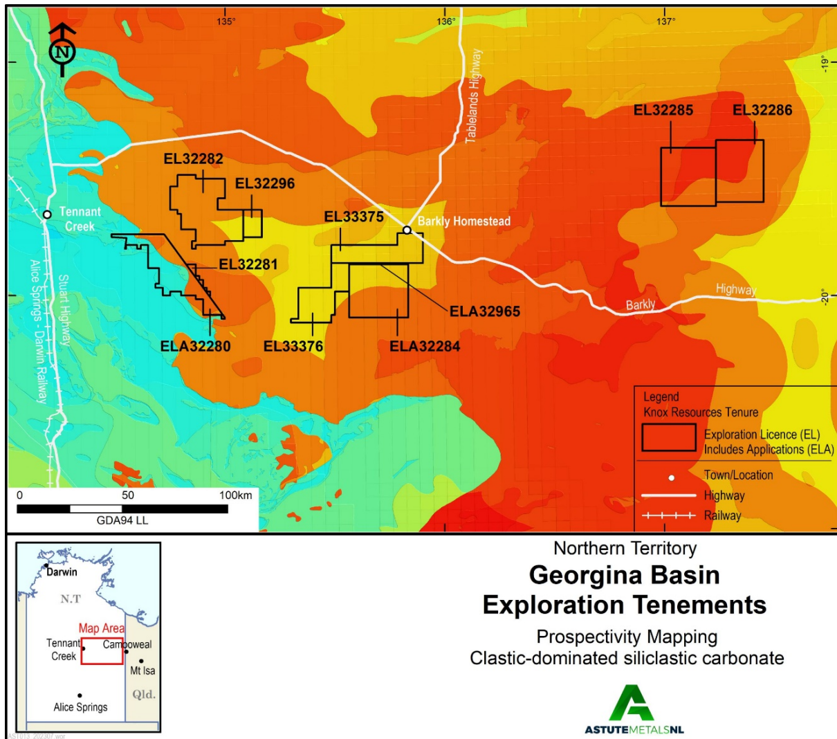
Figure 3. Georgina IOCG Project tenements and Geoscience Australia mineral potential 'heat map', with hotter colours more prospective – noting the Ranken Project tenements EL32285 and EL32286 to the far east of the project.
