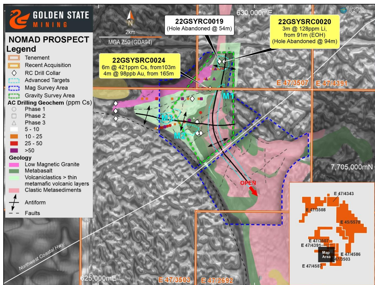
Figure 6: Nomad prospect summary plan showing geophysical survey areas
