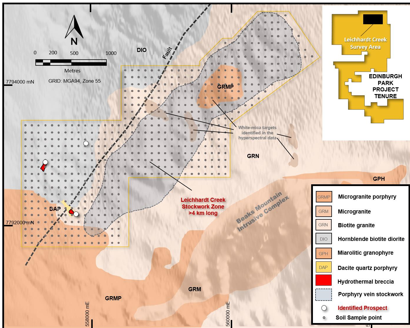
Figure 1: Soil Survey at the Leichhardt Creek Prospect, including simplified geology.
