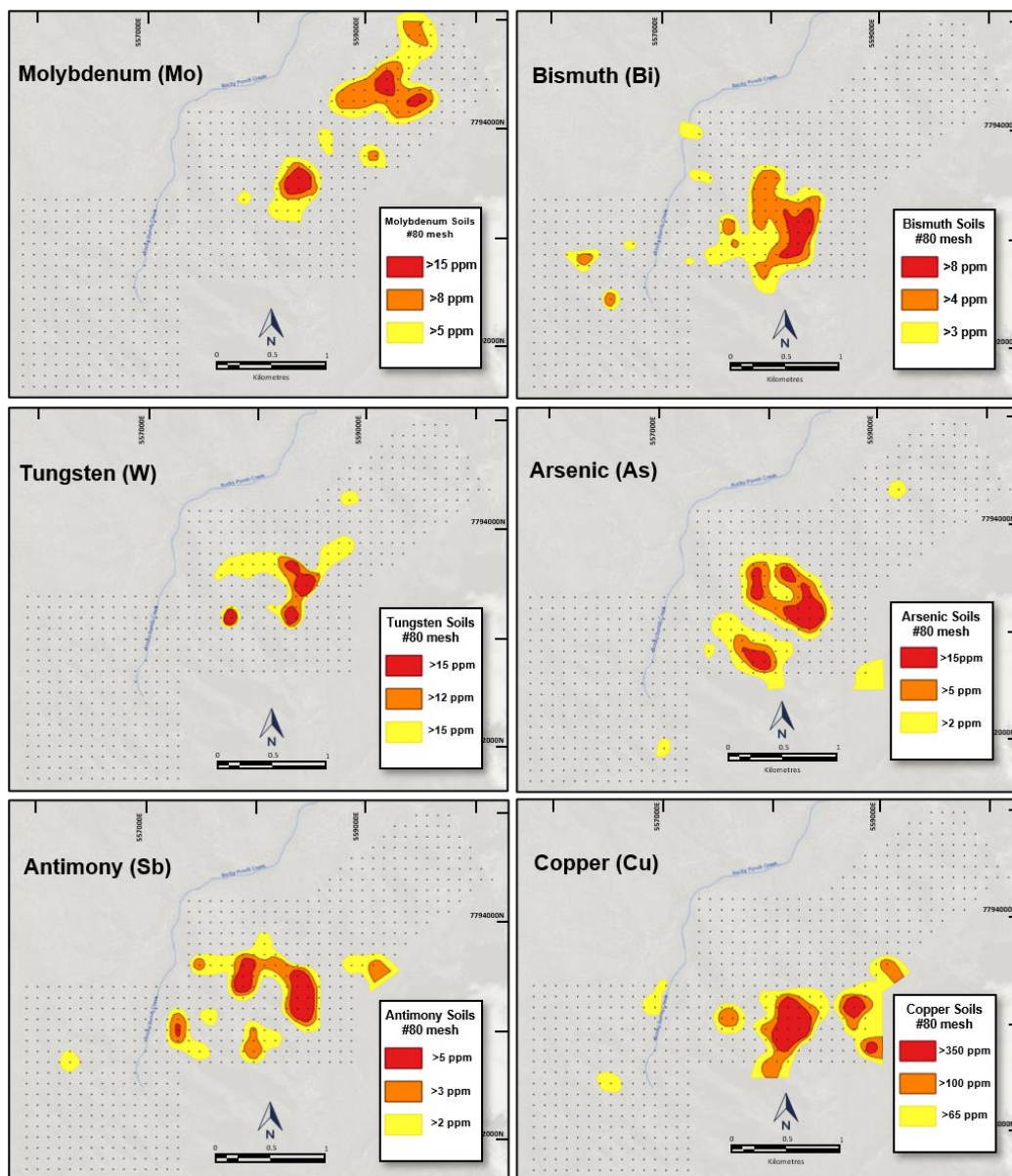
Figure 2: Soil Survey results for Mo, Bi, W, As, Sb & Cu, at the Leichardt Creek Prospect (anomalous pathfinder elements 90th percentile).
