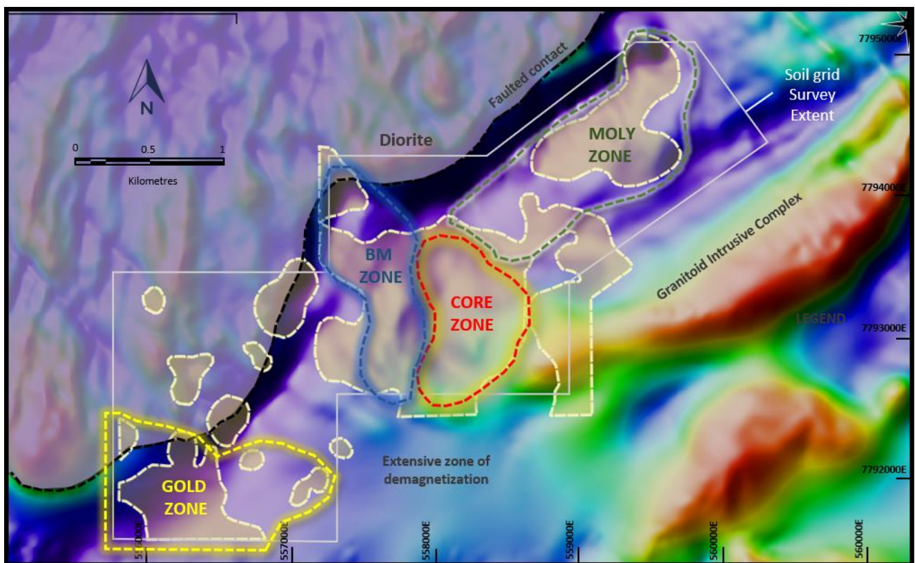
Figure 10: Anomalous geochemistry zones at the Leichhardt Creek draped over RTP magnetic image
