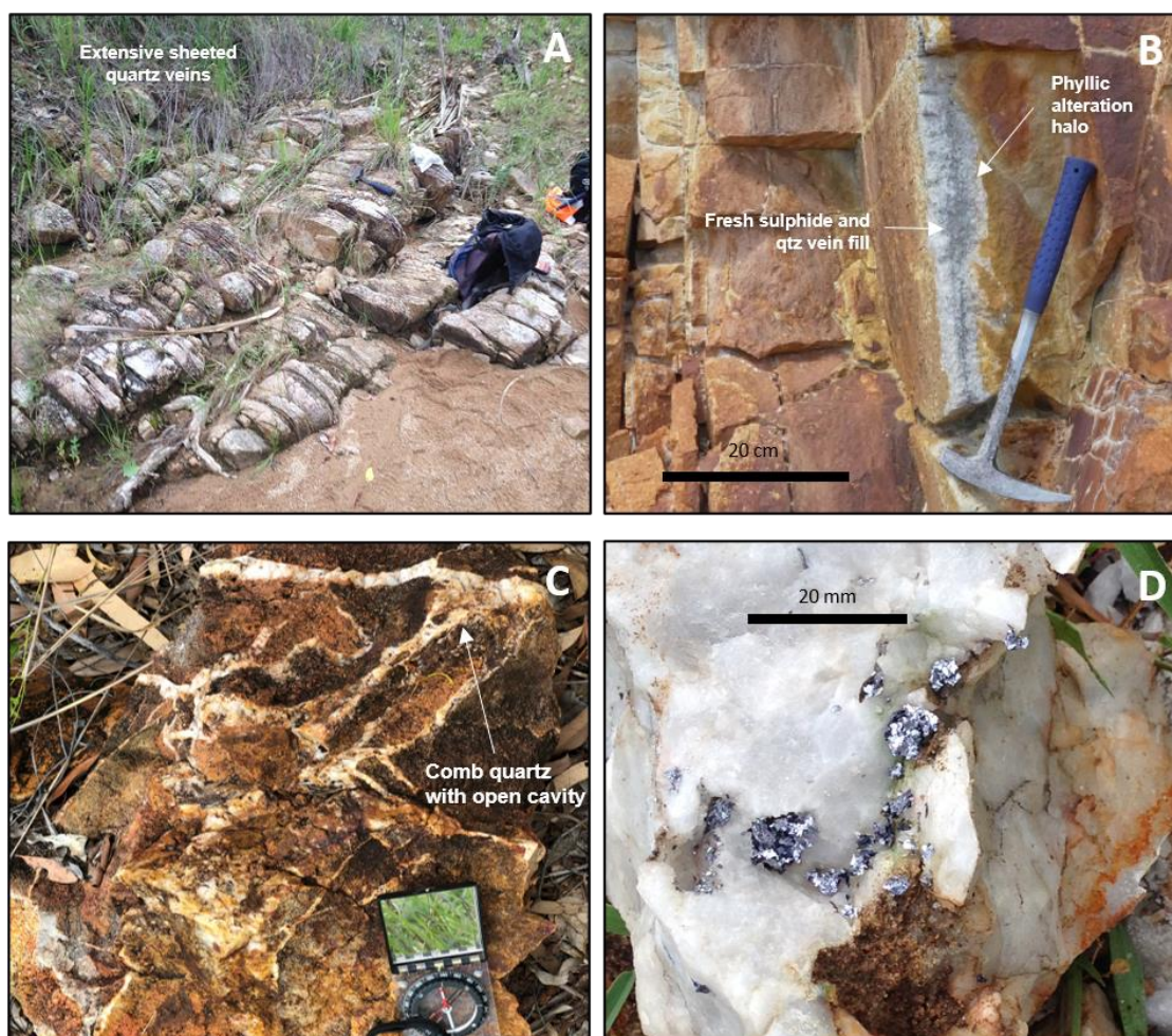
Figure 9: Outcrop and Sampling at the Leichardt Creek
