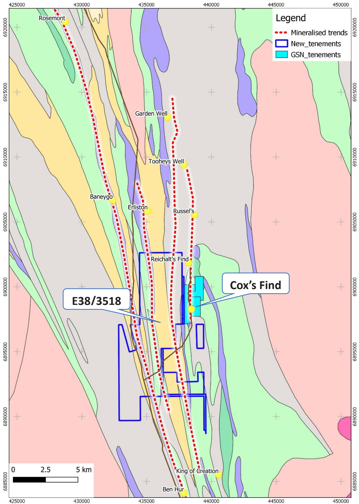
Figure 1: Plan view of the Cox's Find Project (light blue) and the applications lodged (dark blue) highlighting mineralised trends (red dashed lines) with GSWA geology background
