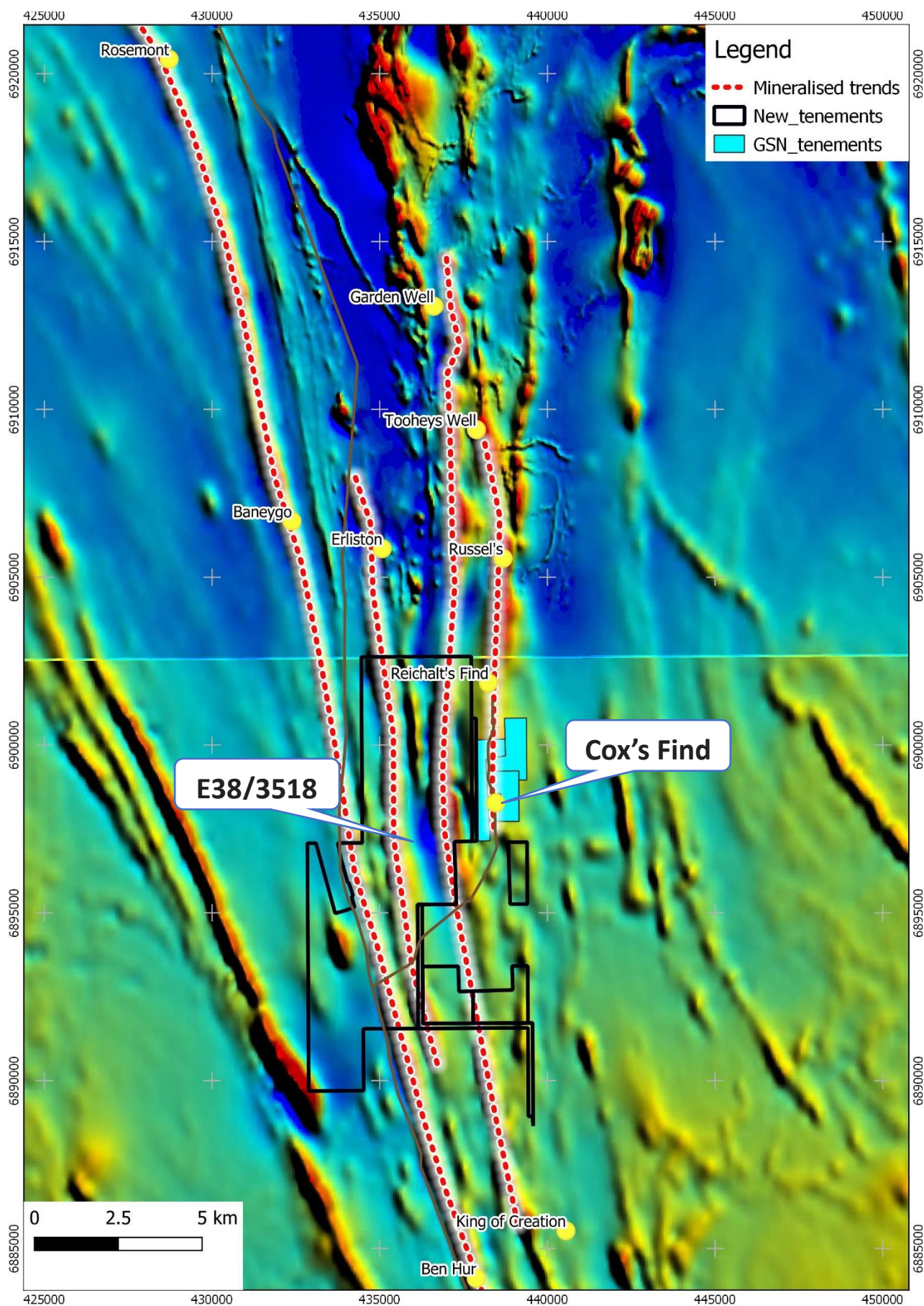
Figure 2: Plan view of the Cox's Find Project (light blue) and the applications lodged (black outline) highlighting mineralised trends (red dashed lines) with GSWA magnetic data (TMI) background.
