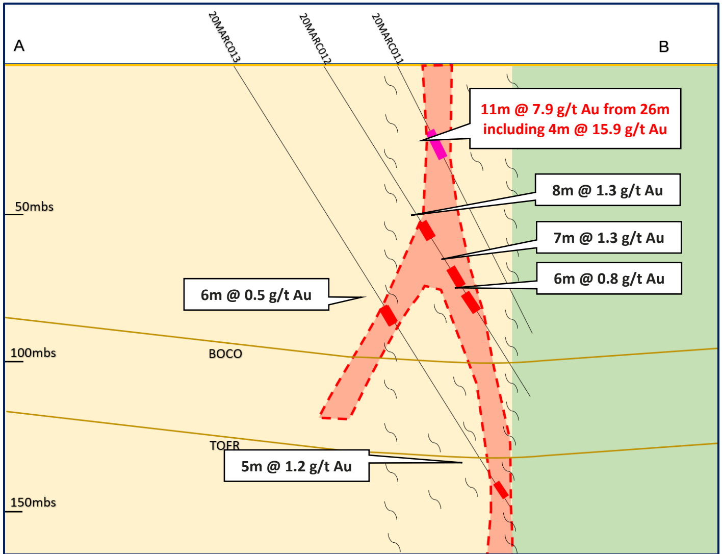
Figure 2: Section A-B view of the Mon Ami Gold Project highlighting the location of recent high-grade intercepts at the intersection of NE splays and the sheared mineralised contact of the sedimentary package (pale yellow) and the basalt unit (green).
