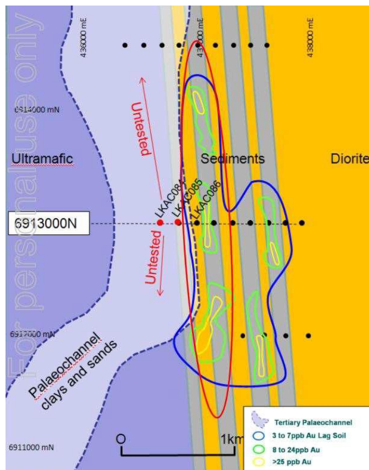
Figure 2. Gold-in-soil results from Garden Well for context. The figure shows that a 3 ppb anomaly was used to illustrate Garden Well after its discovery with contour values of 8 ppb to 24 ppb and greater than 25 ppb. Refer to Regis Resources presentation release dated 8 February 2010.
