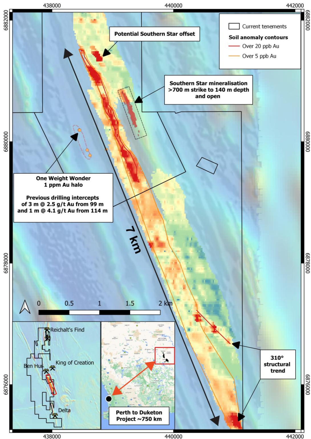
Figure 1. Geochemical heat map showing gold anomalism from a recent soil survey underlain by aeromagnetic imagery. Results of the recent survey, conducted along a stratigraphic trend west of the main Southern Star prospect, have been merged with previous geochemical surveys in the area, showing a distinct 7 km anomalous trend. The image also shows the One Weight Wonder prospect and another geochemical gold anomaly to the north of Southern Star, which may be a fault offset of the main Southern Star mineralisation.
