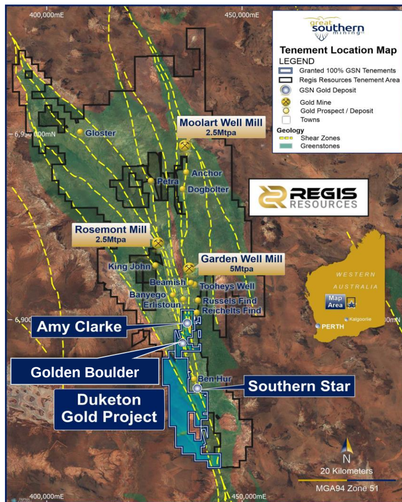
Figure 3. Plan view of GSN's tenement holding in the Duketon Gold Belt highlighting the locations of prospects and proximity to Regis' Garden Well, Rosemont and Moolart Well mills. Mineralised gold trends are delineated in yellow.
