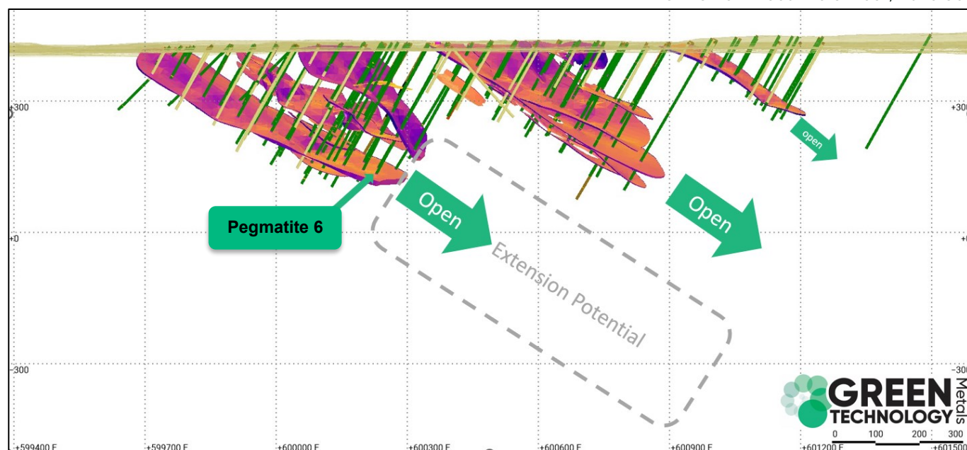
Figure 1: Stacked LCT pegmatites at Root Bay with mineralised defined from surface to 300m depth, and open.
