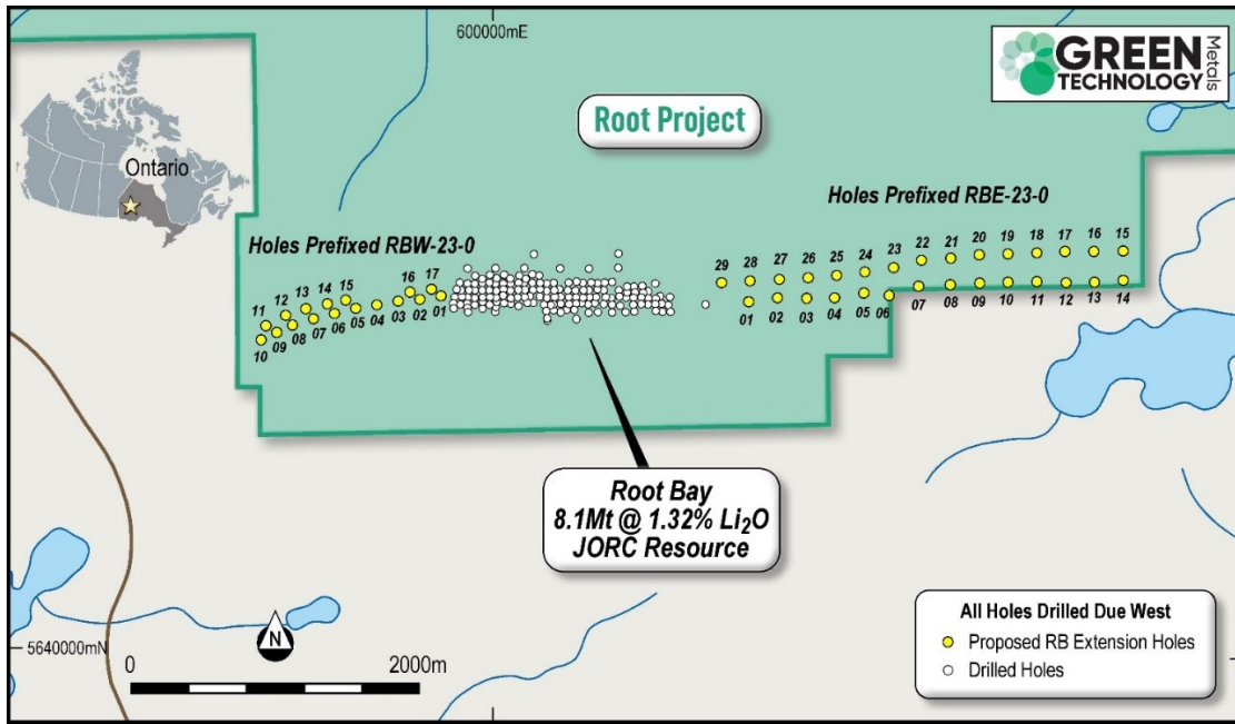
Figure 2: Root Bay, phase 2 extensional drill plan
