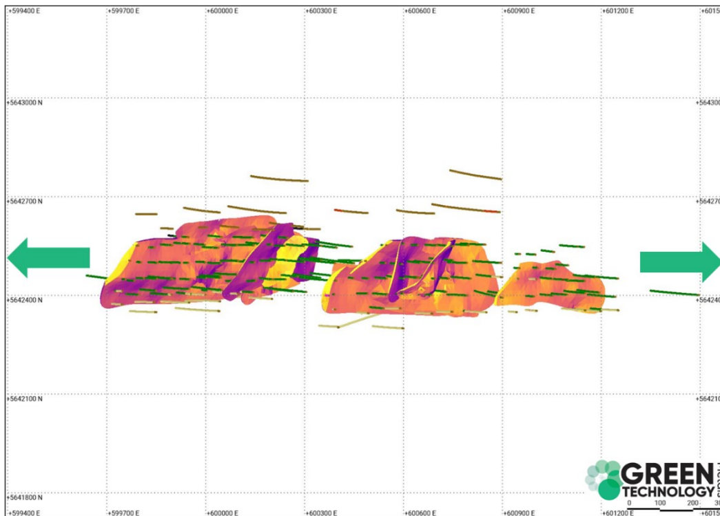
Figure 3: Root Bay Ridge potential for stacking to continue
