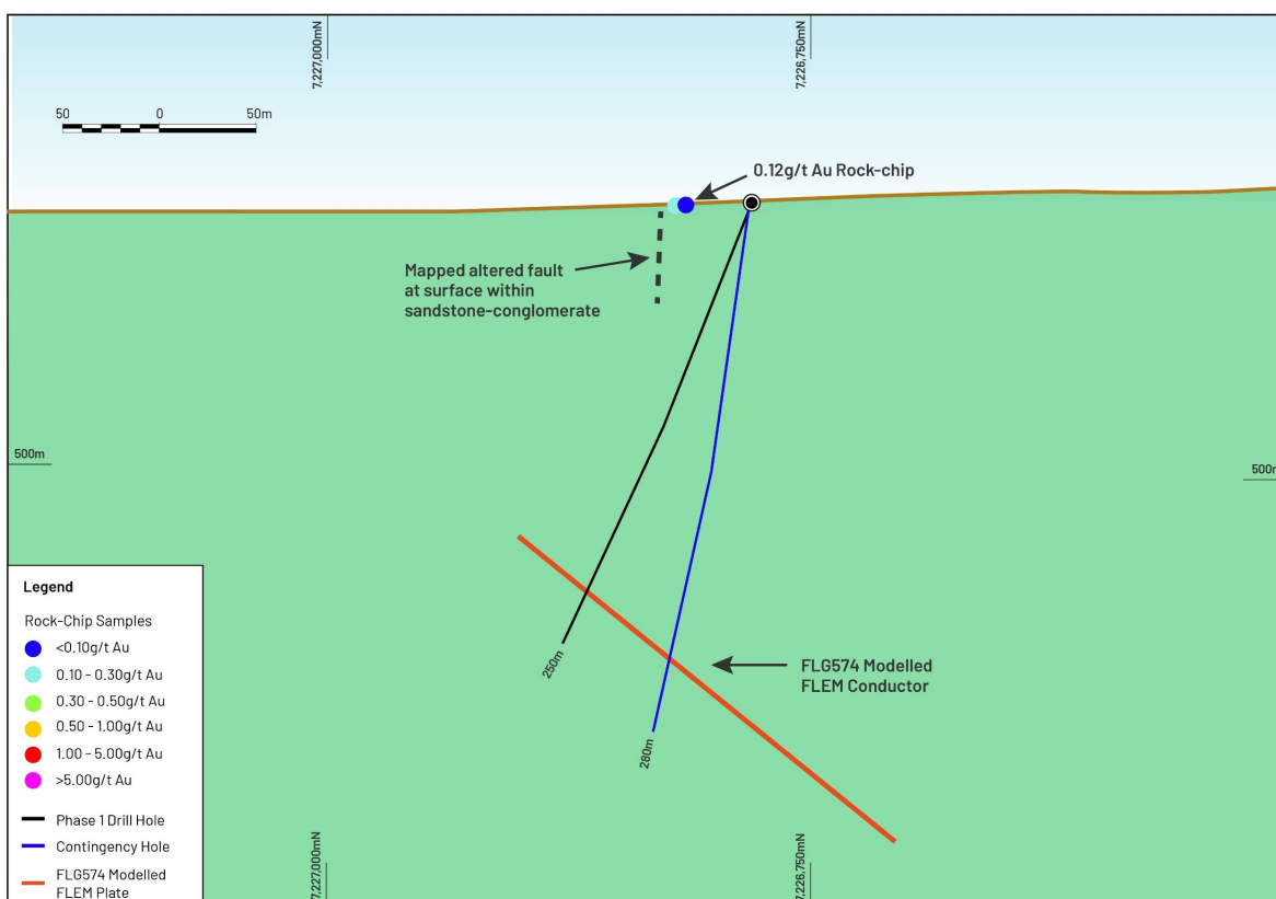
Figure 5: FLG574 modelled plate FLEM conductor, with designed drill-holes to test for VHMS mineralisation. The Plate has extents of approximately 480m x 170m and is within 190m of surface.
