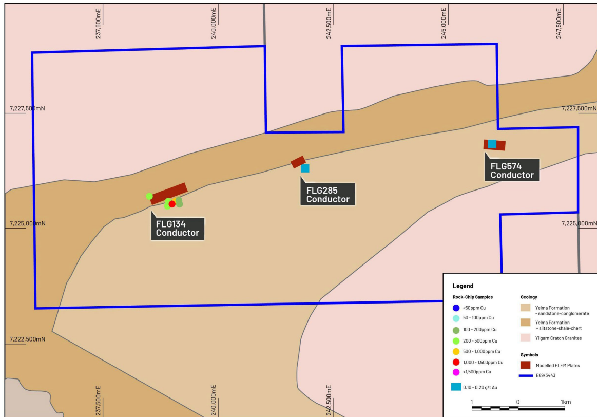
Figure 2: Plan location of modelled FLEM conductors FLG134, FLG285, and FLG574 (GTE ASX Announcement 26 September 2023).
