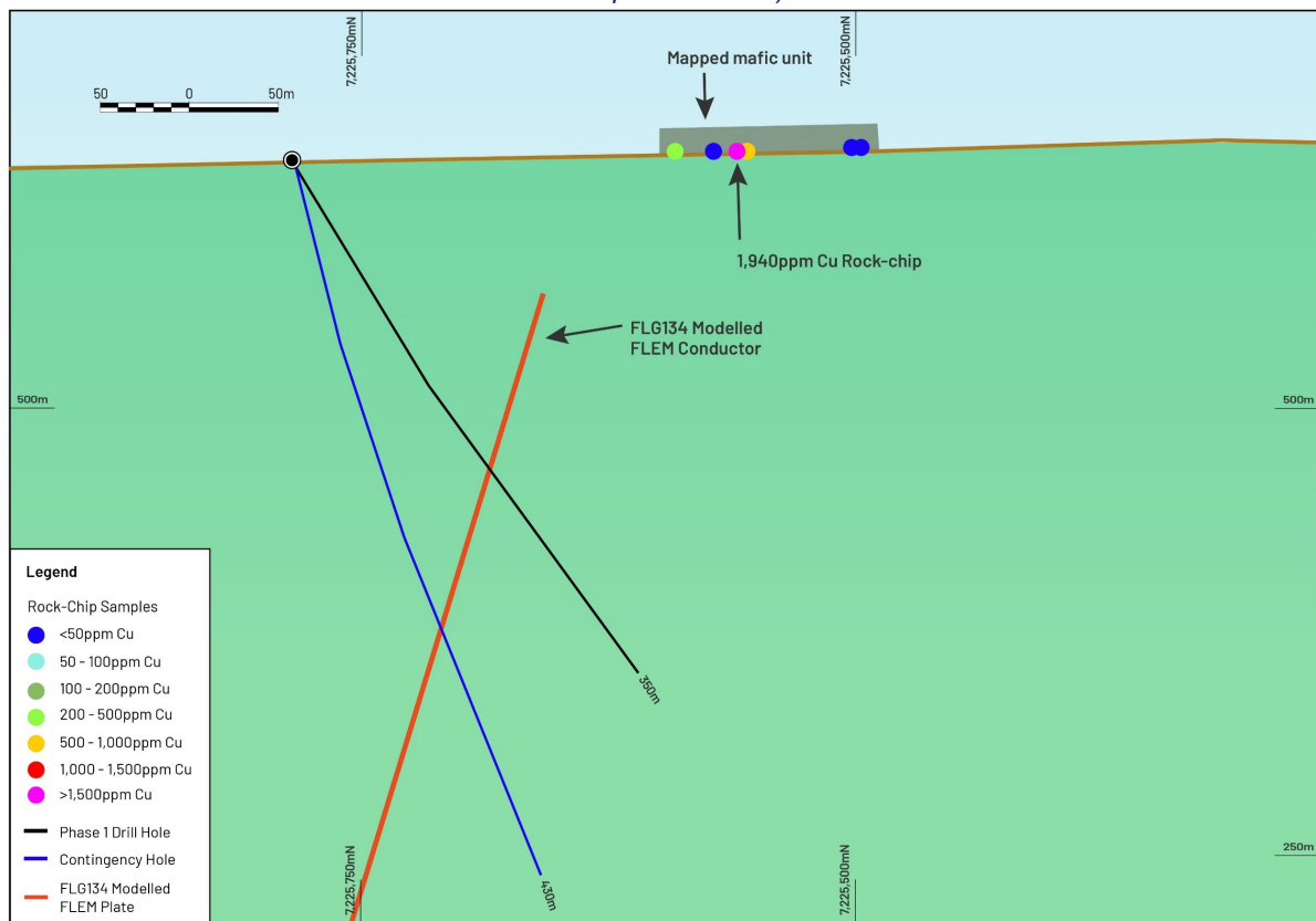
Figure 3: FLG134 modelled plate conductor and designed drill-holes to test for VHMS mineralisation. Plate FLG134 has extents of 800m x 600m, with the top of the plate within 80m from surface.
