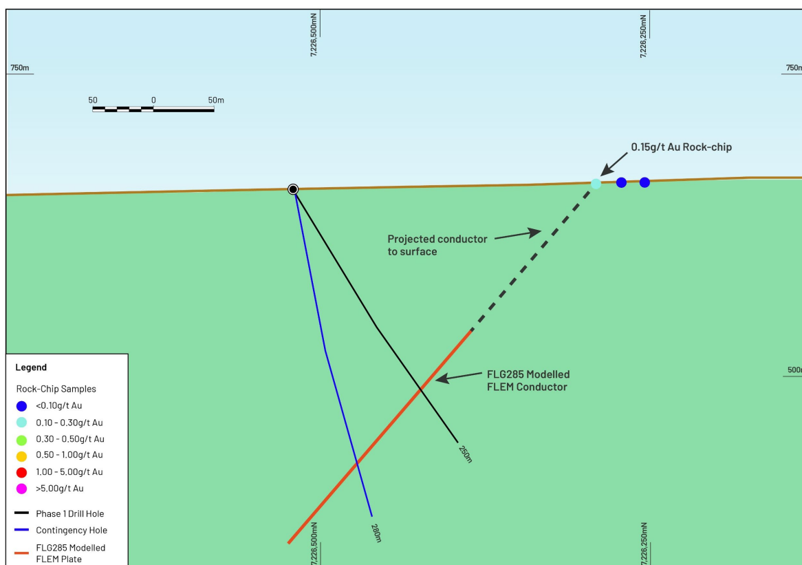
Figure 4: FLG285 modelled plate FLEM conductor, with designed drill-holes to test for VHMS mineralisation. The plate has extents of approximately 280m x 180m and is within 120m of surface.
