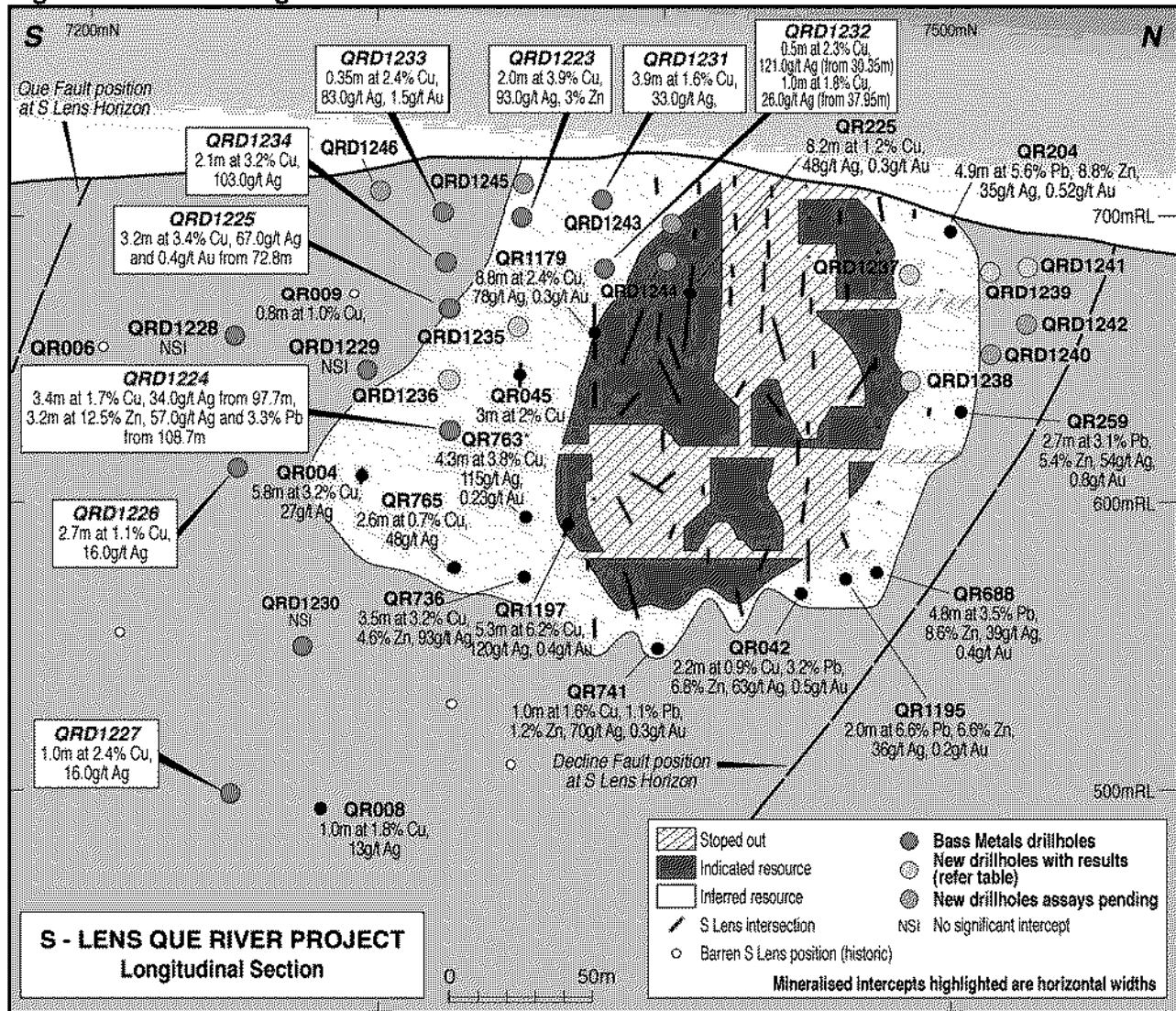
Figure 1: S-Lens Long Section
