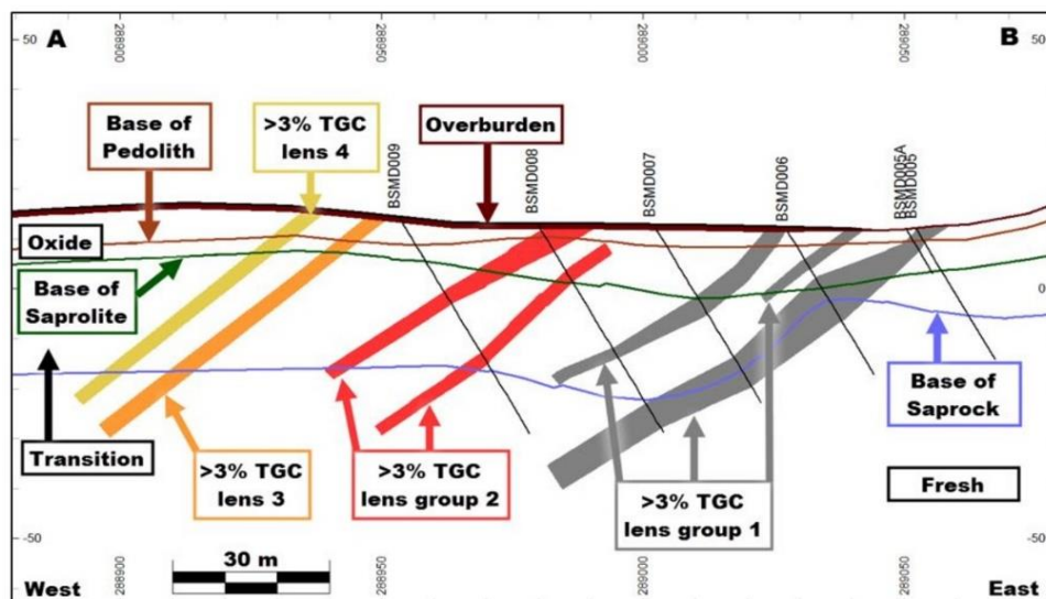
Figure 2. Cross section of the northern mineralization zone at the Mahefadok prospect.
