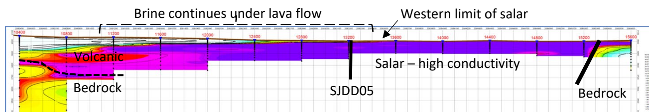
Figure 9: Cross section along TEM line 6, showing the extension of brine (pink to blue zones) beneath lava flows west of the salar
