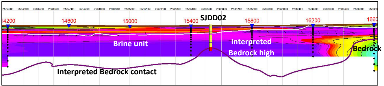
Figure 3: TEM profile around hole SJDD02, showing the conductive zone (pink and blue) and interpreted bedrock (yellow). The section looking towards the north. Pink intervals on the drill hole are volcanics, yellow are clastic sediment units, grey are breccia units, red metamorphosed sediments (bedrock). The drillhole is projected onto TEM Section 1, 7019000 North, showing Eastings in the GK2 coordinate system.
