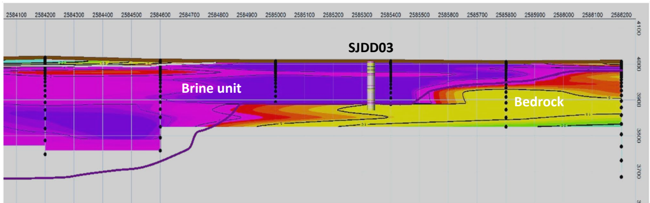
Figure 5: TEM profile around hole SJDD03, showing the conductive zone (blue to pink) and interpreted bedrock. Section looking towards the north. Pink intervals on the drill hole are volcanics, yellow are clastic sediment units, grey are breccia units. The base of the hole intersects laminated siliceous metamorphosed sediments (bedrock). The drillhole is projected onto TEM Section 3, 7017000 North, showing Eastings in the GK2 coordinate system.
