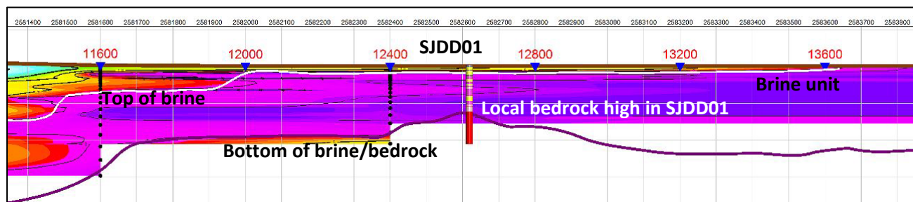
Figure 2: TEM profile around hole SJDD01, showing the conductive zone (blue to pink) and interpreted bedrock. Section looking towards the north. Pink intervals on the drill hole are volcanics, yellow are clastic sediment units, grey are breccia units, red are metamorphosed sediments (bedrock). This is TEM Section 2, 7018000 North, showing Eastings in the GK2 coordinate system.
