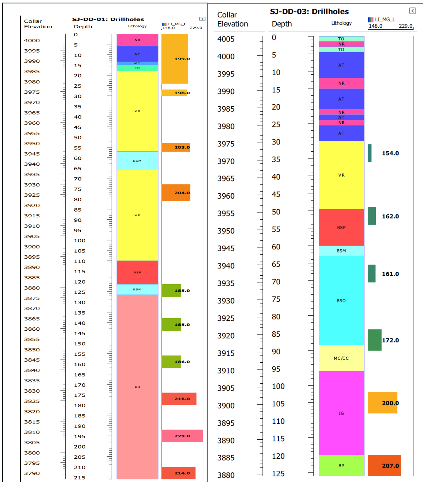
Figure 2: SJDD01 and SJDD03 lithology, packer sampling depths and assays. The upper section of SJDD01 is principally basalt (VR), and the lower part of the hole fractured basement rock (BB). Hole SJDD03 is composed of volcanic ashes and reworked volcanic material (matrix supported clastic material of volcanic origin), overlying metasedimentary bedrock (BP).
