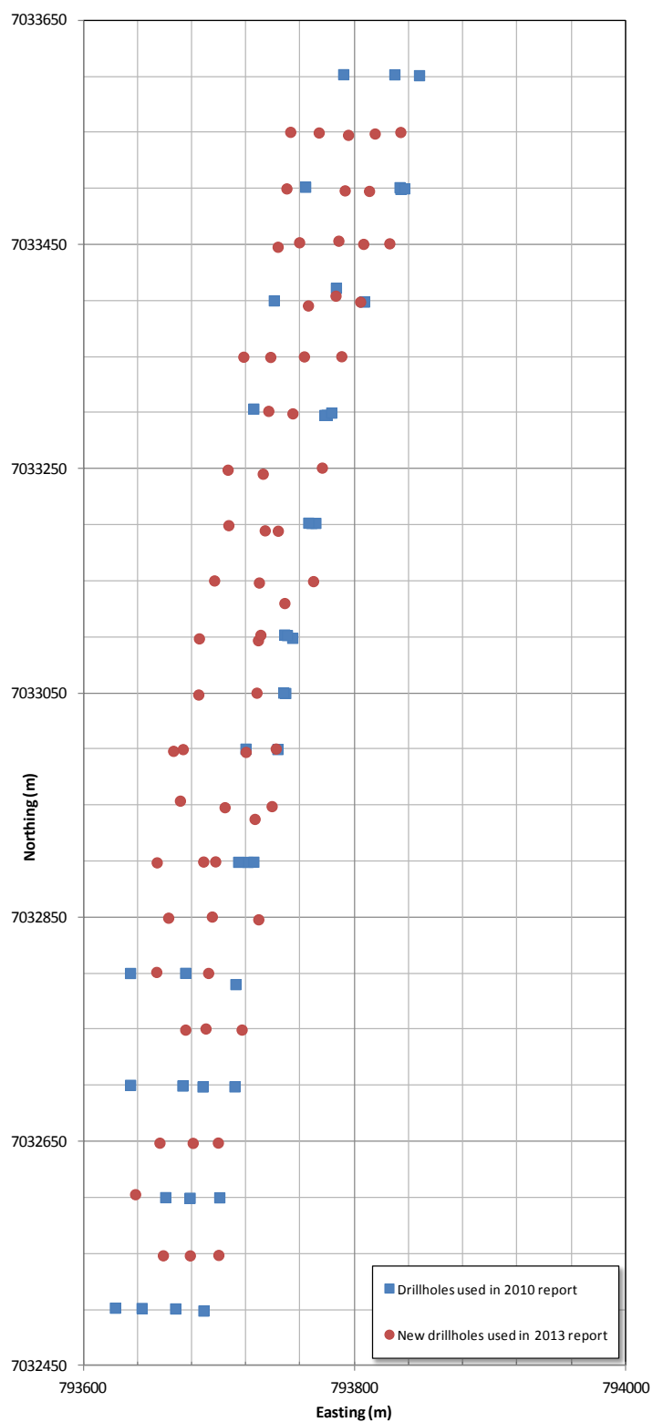
Figure 2 – JWD deposit drill hole collar location plan (blue – drilled prior to 2010 Mineral Resource, red – drilled after that time)
