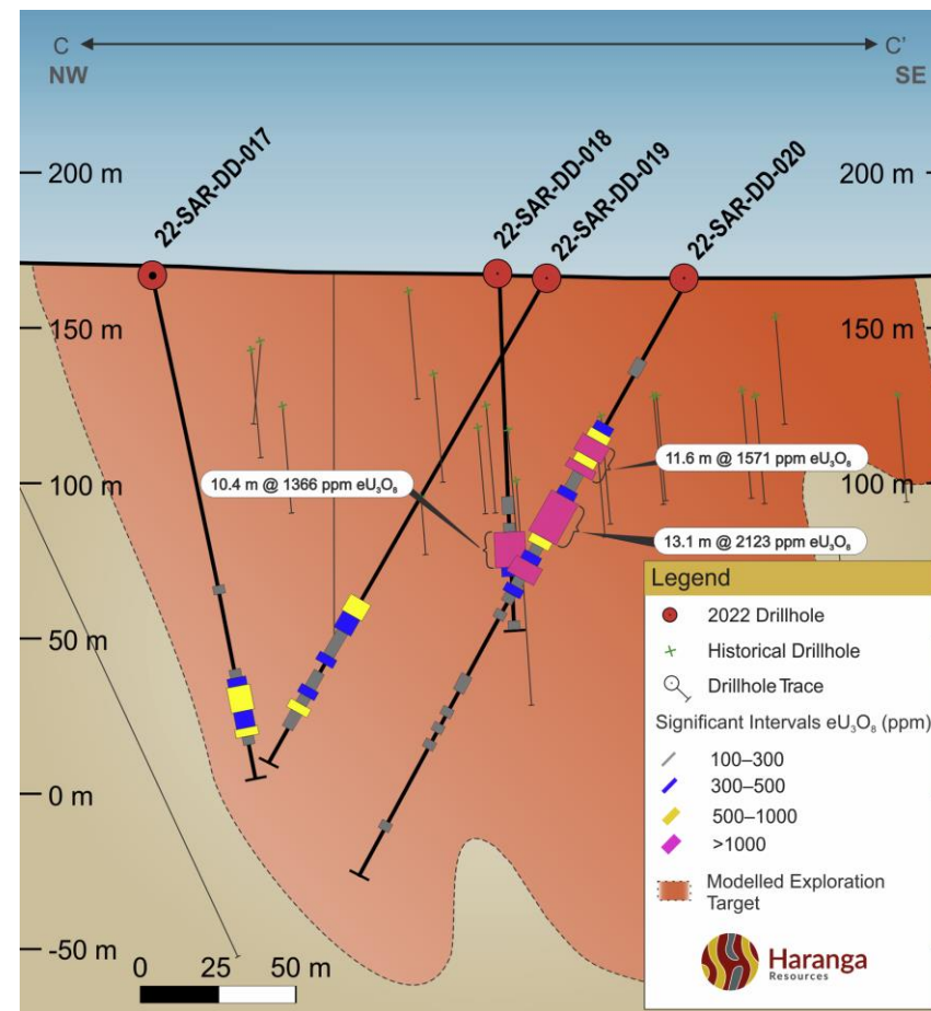
Figure 6: Cross-section C-C'. See Figure3 for the location of the section line.
