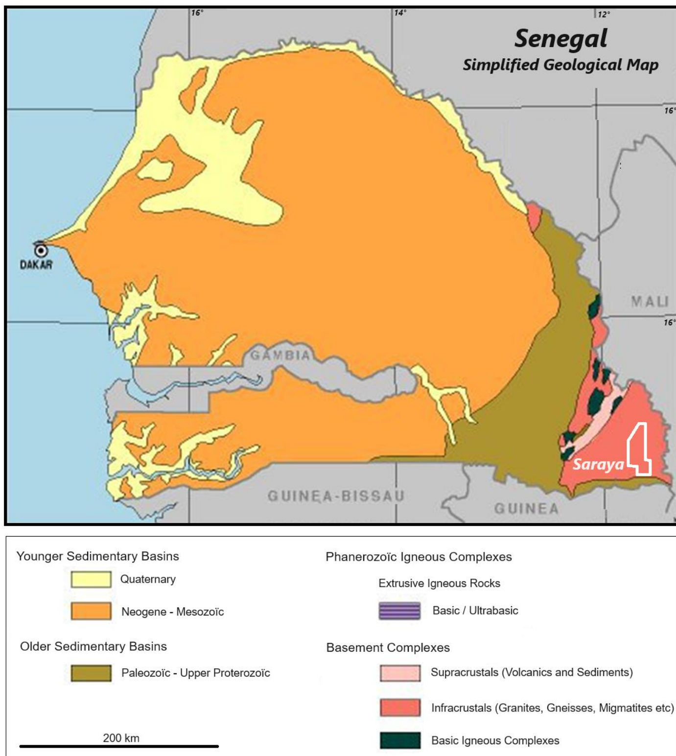
Figure 2: Senegal Geology
