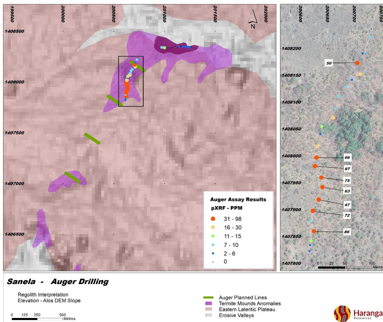
Figure 4: Location and assay results of the first auger drilled line at the Sanela Prospect 3 . The assay results in the saprolite below the lateritic cover range from 47ppm to 97 ppm uranium (pXRF).
