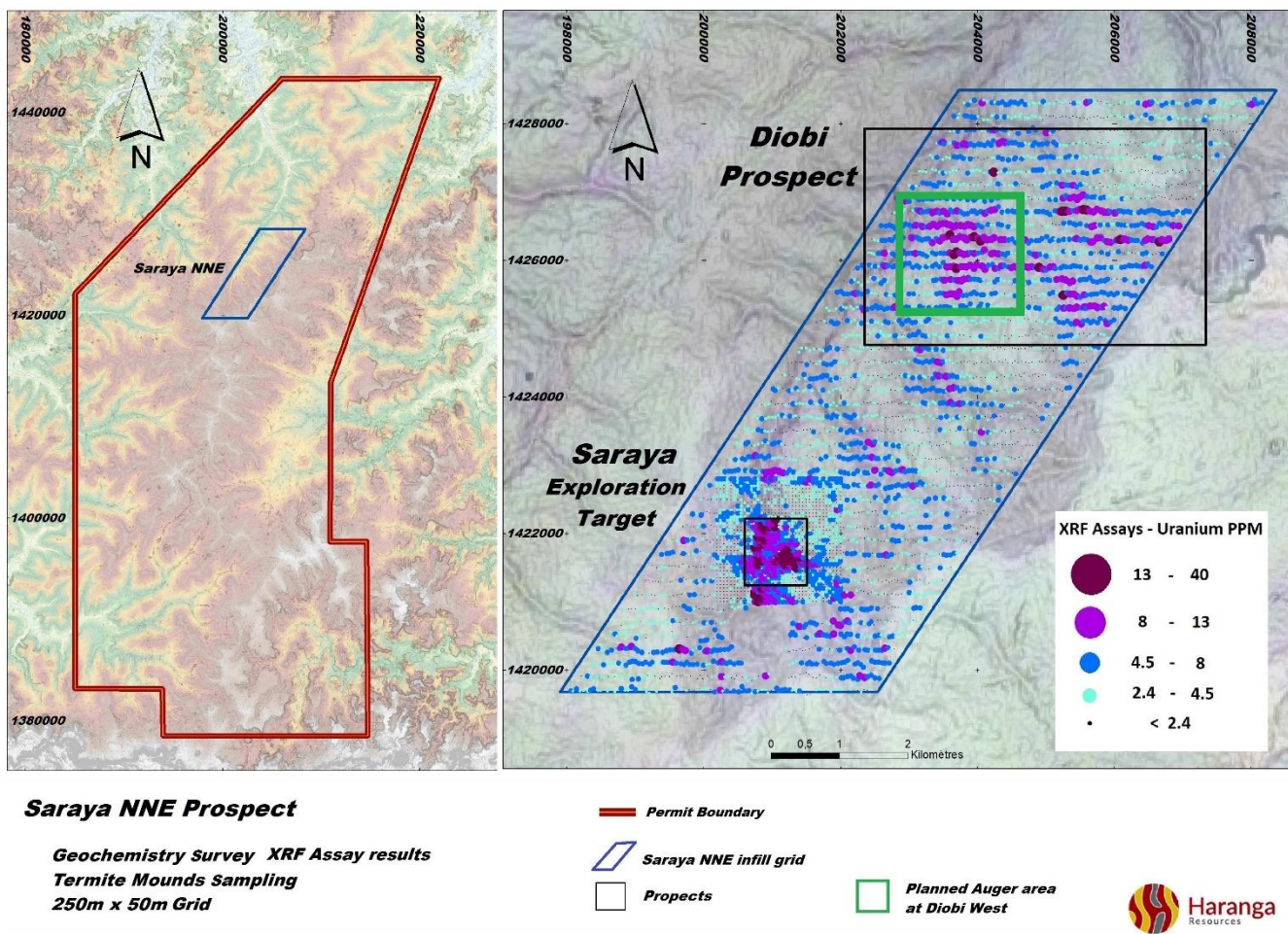
Figure 5: Location of the planned auger drilling target area over the Diobi prospect in the Saraya NNE termite-mound infill grid (All results displayed – pXRF) 2 .
