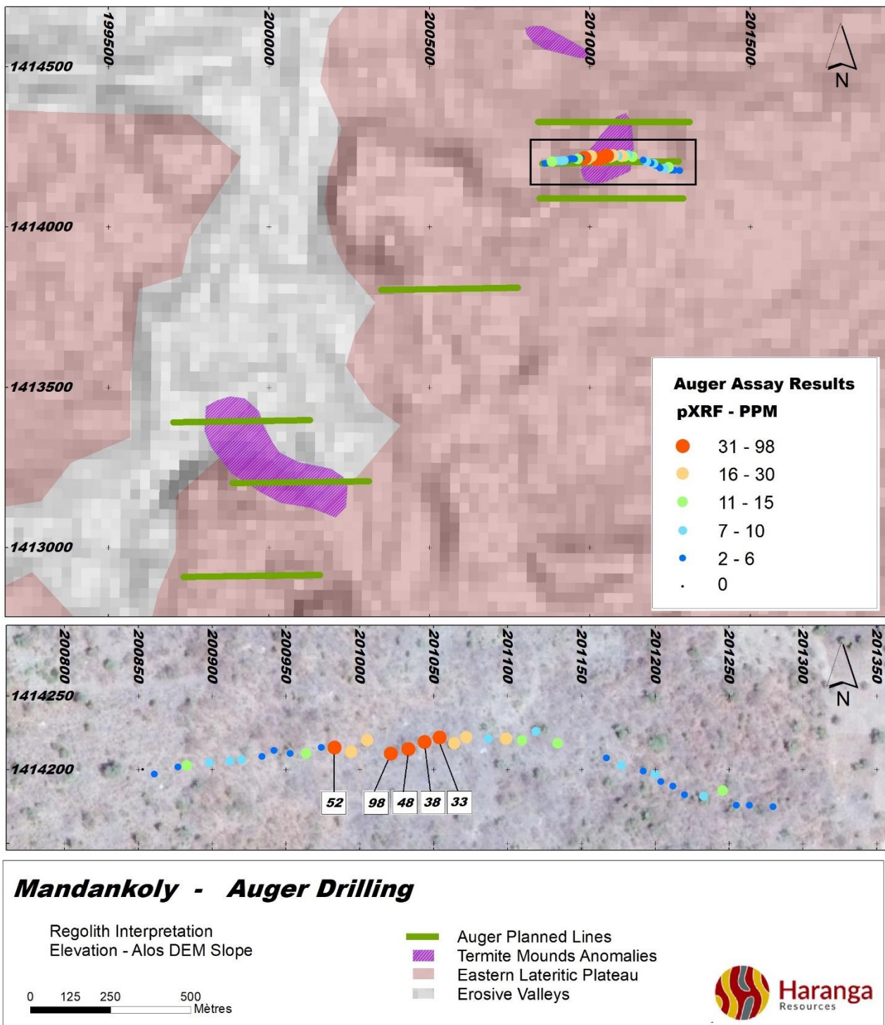
Figure 2: Location of the completed auger line at Mandankoly, over the termite mound anomaly 4 , and planned auger lines. Bottom window is the detail of the drilled line.
