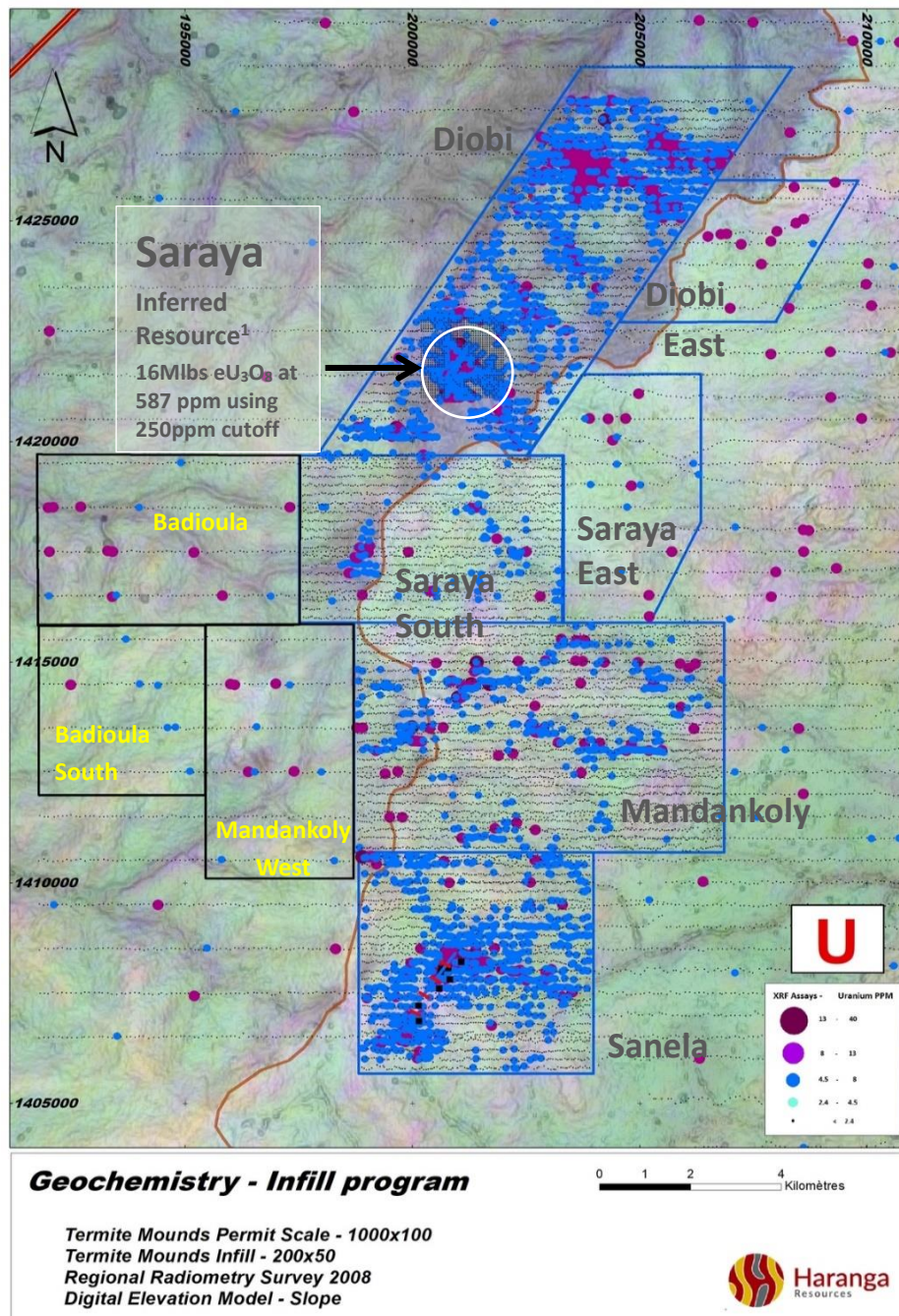
Figure 1: Location of the termite mound infill sampling grids and pXRF results to date.
