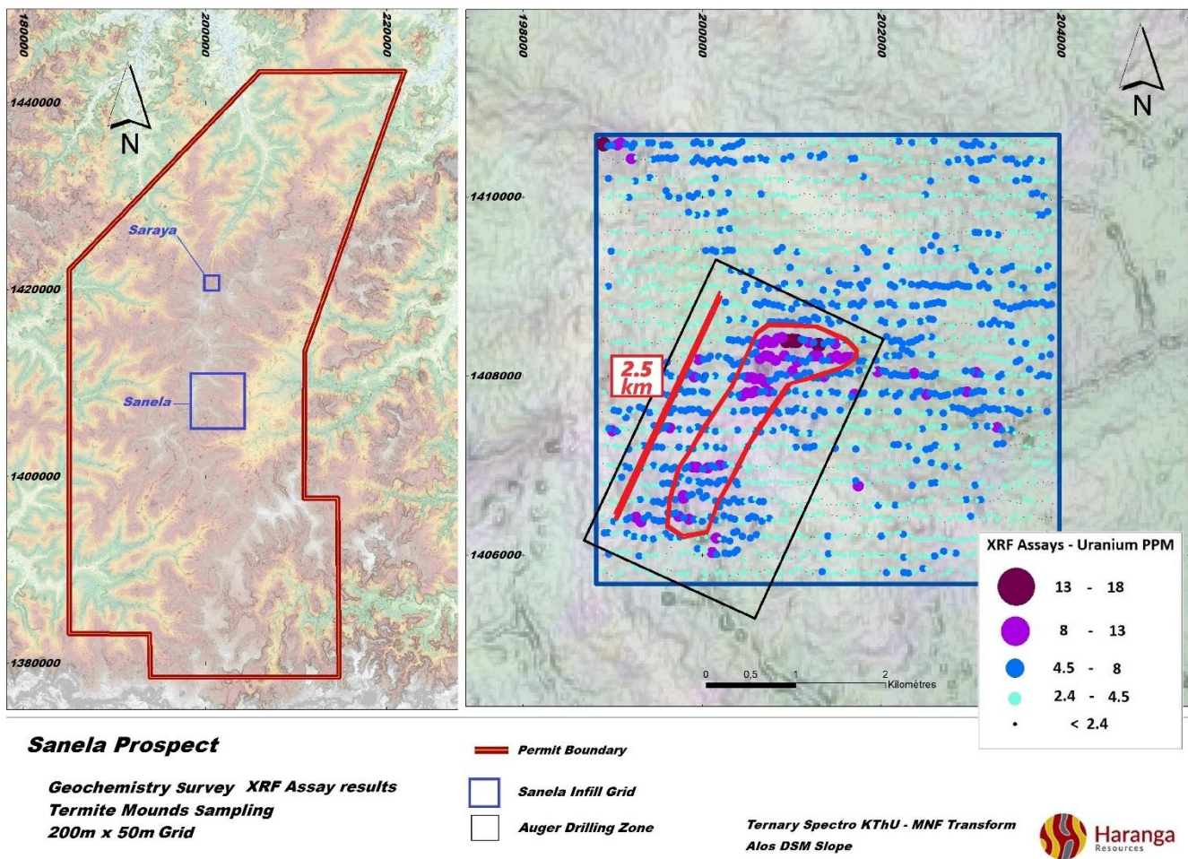
Figure 3: Location of the Sanela NNE trend with termite mound uranium concentrations (pXRF) and auger drilling target zone at the Sanela Prospect 3 .
