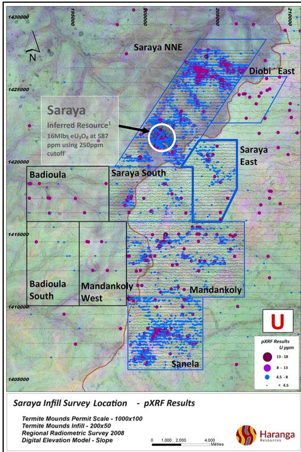
Figure 1: Location of the termite mound infill sampling grids and pXRF results to date 123 .
