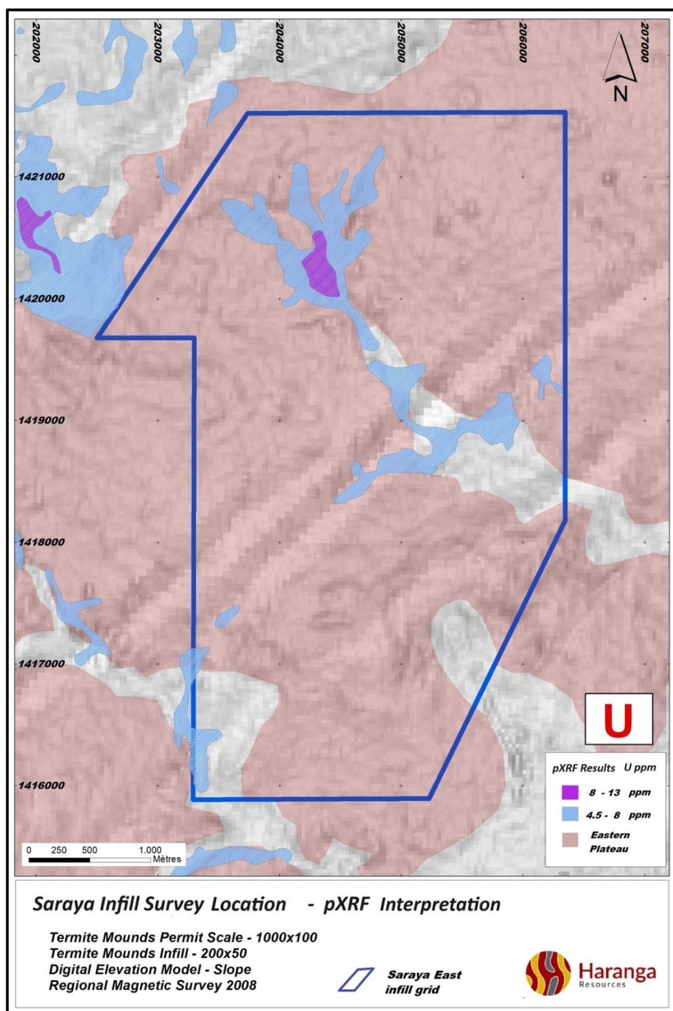
Figure 3: Saraya-East anomaly over Eastern Lateritic Plateau.
