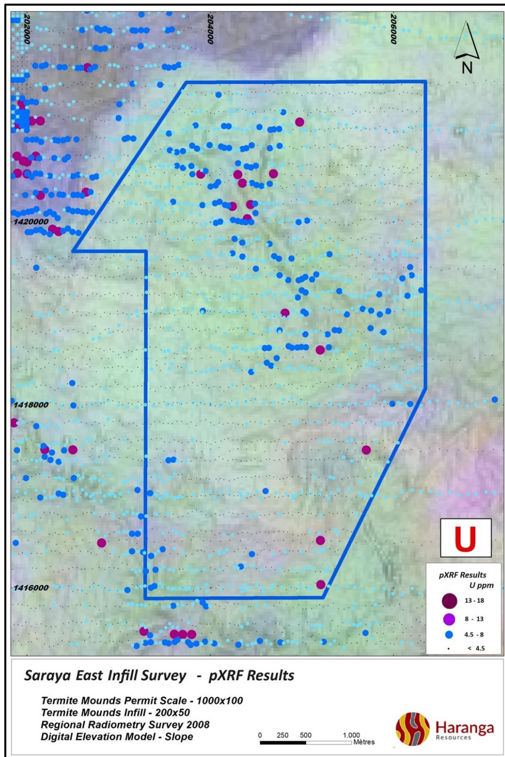
Figure 2: pXRF results of the Saraya-East infill sampling.
