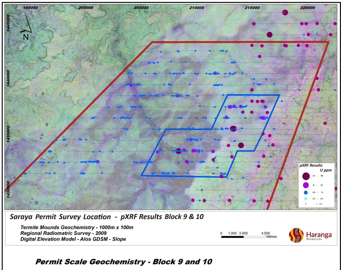
Figure 4: Location and TMS uranium concentrations (pXRF) in Blocks 9 and 10. The area outlined in blue will be covered with 200m x 50m TMS in-fill sampling.
