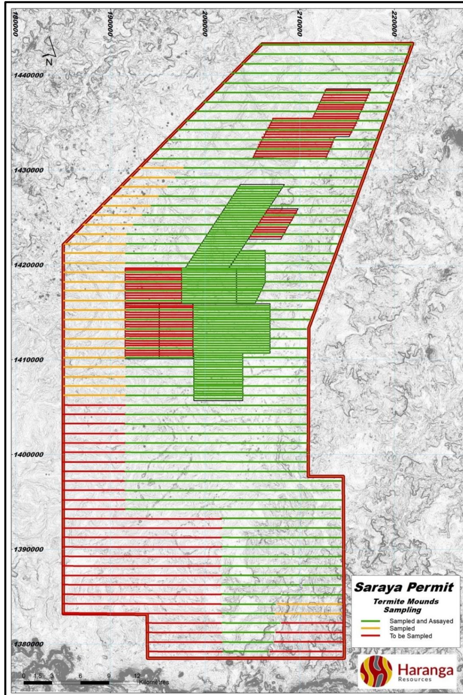
Figure 5: Termite mound sampling progress at Saraya.
