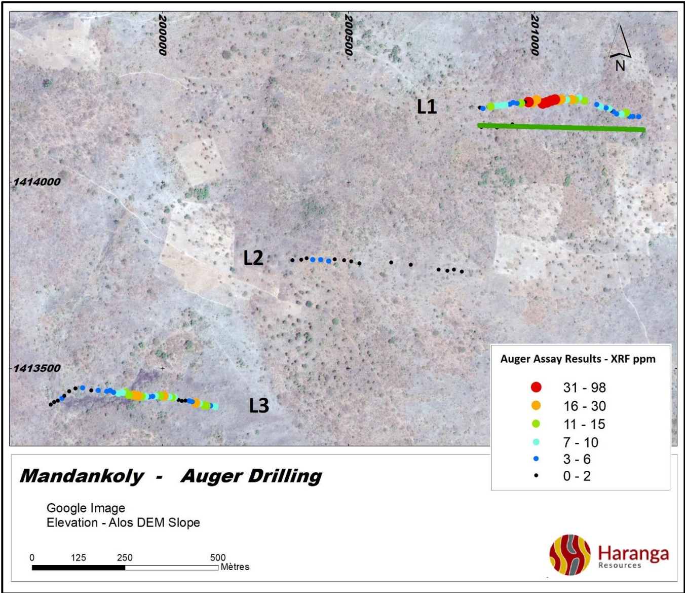
Figure 6: Location of the Auger lines L1, L2 and L3 with pXRF results and the new line being drilled immediately south of the anomalous zone discovered on Line 1 5 .
