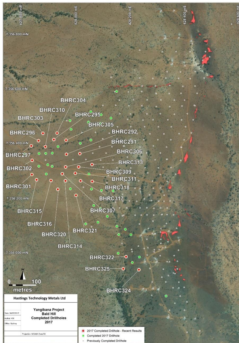
Figure 2 – Yangibana Project, Bald Hill, 2017 Drilling, Recent Results
