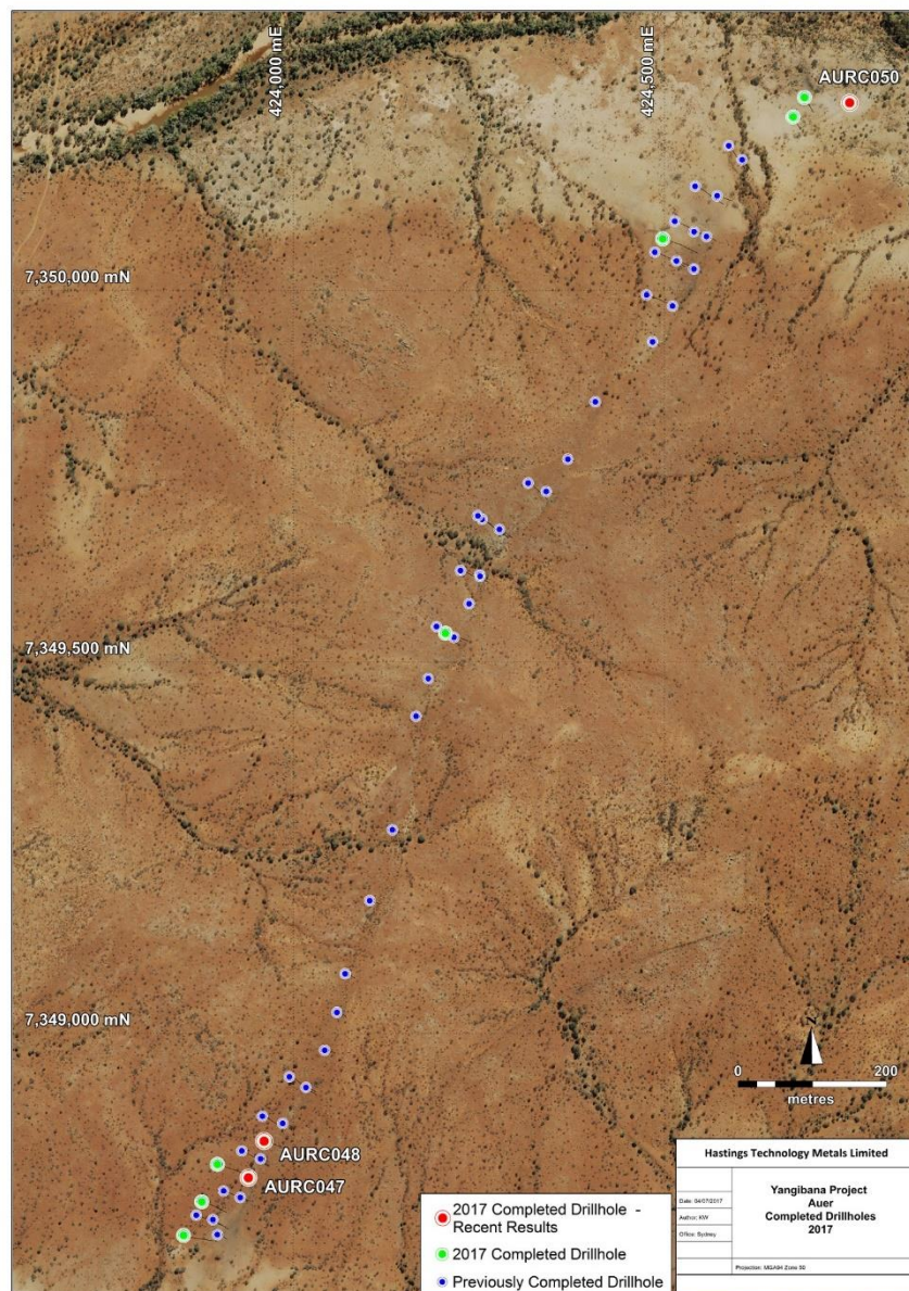
Figure 4 – Yangibana Project – Auer, 2017 Drilling, Recent Results
