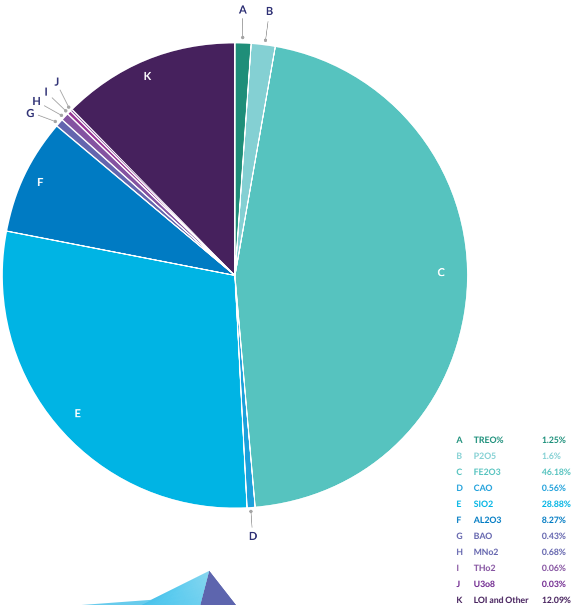
Ore Composition Chart
