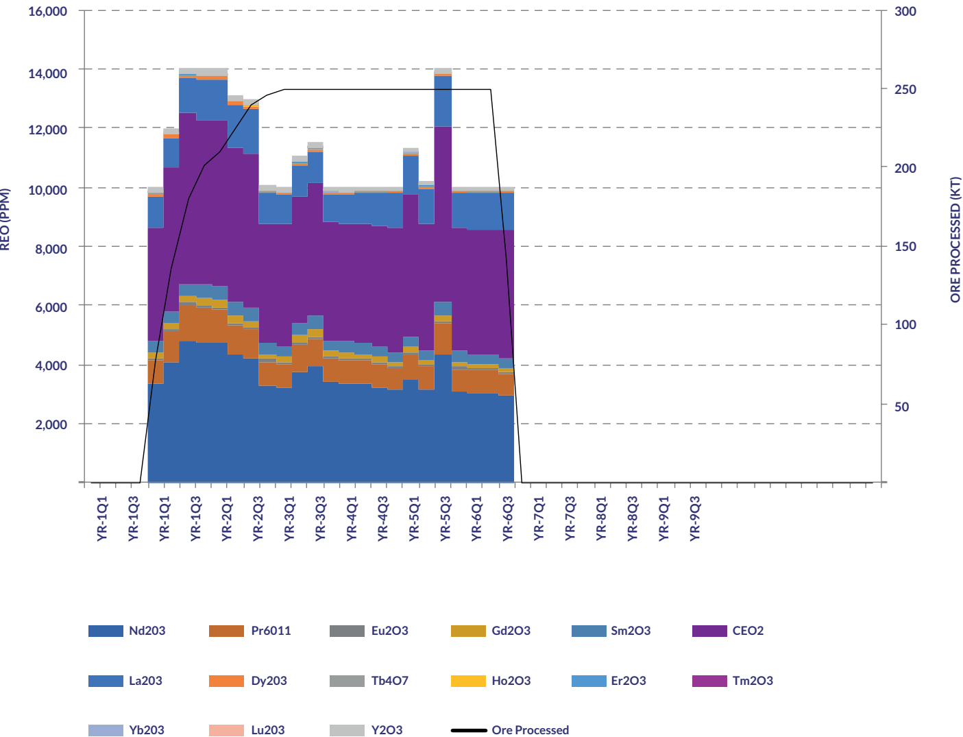
Figure 5-4: Ore Processing
