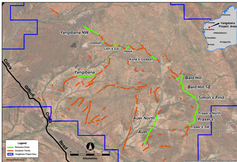
Figure 1: Exploration Target
