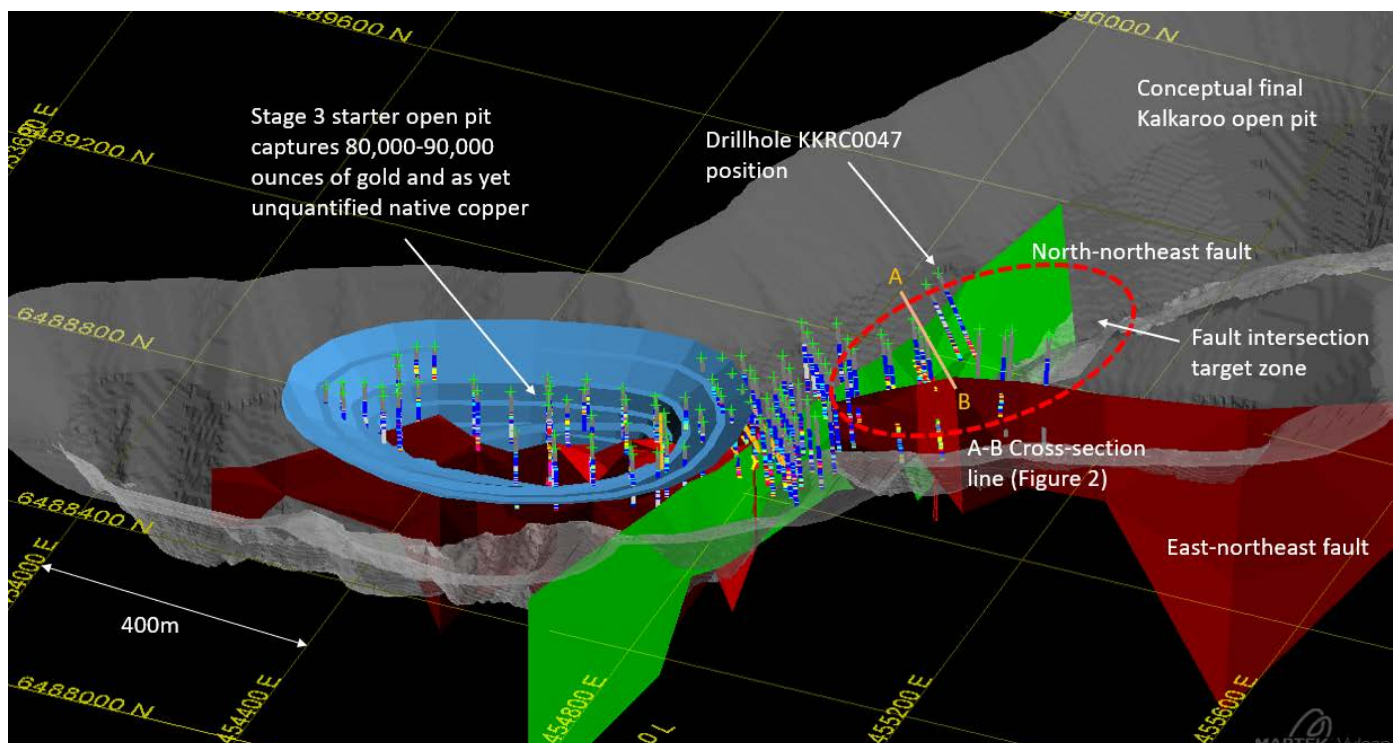
Figure 1 Recent RC drilling at West Kalkaroo is located several hundred metres east of the planned Stage 3 starter open pit (blue), with the Figure 2 cross-section line shown (orange line marked A-B). The target of current drilling (within the dashed red outline area) lies at the intersection zone of two major faults shown in red and green.
