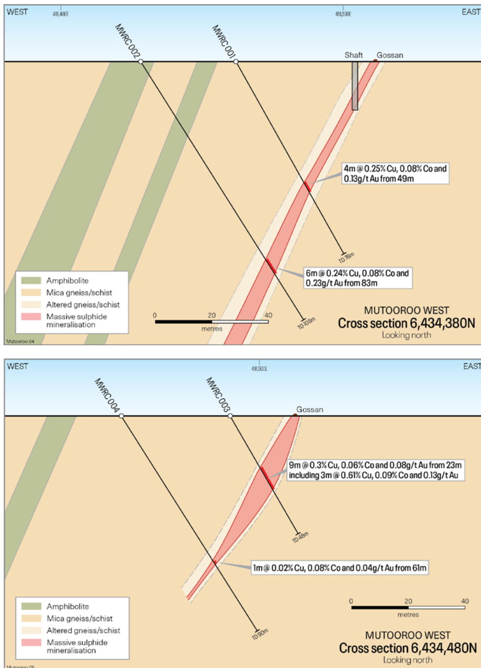
Figures 5 & 6 Drill cross sections through the Mutooroo West lode (see Figure 3 for RC drillhole locations). All holes intersected copper-cobalt-gold mineralisation in a narrow lode position at moderately shallow depths. There remain possibilities for shallow mineralisation along strike and also thicker massive sulphide mineralisation at depth, given the significant AEM geophysical anomaly in the vicinity.
