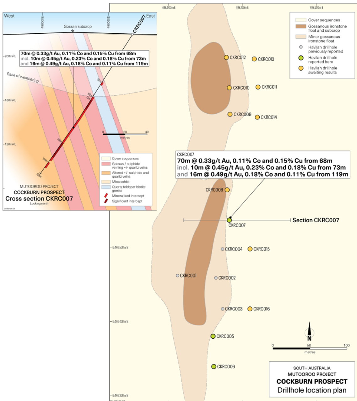
Figure 5 Location of drillhole CKRC007 and cross section at Cockburn prospect.
