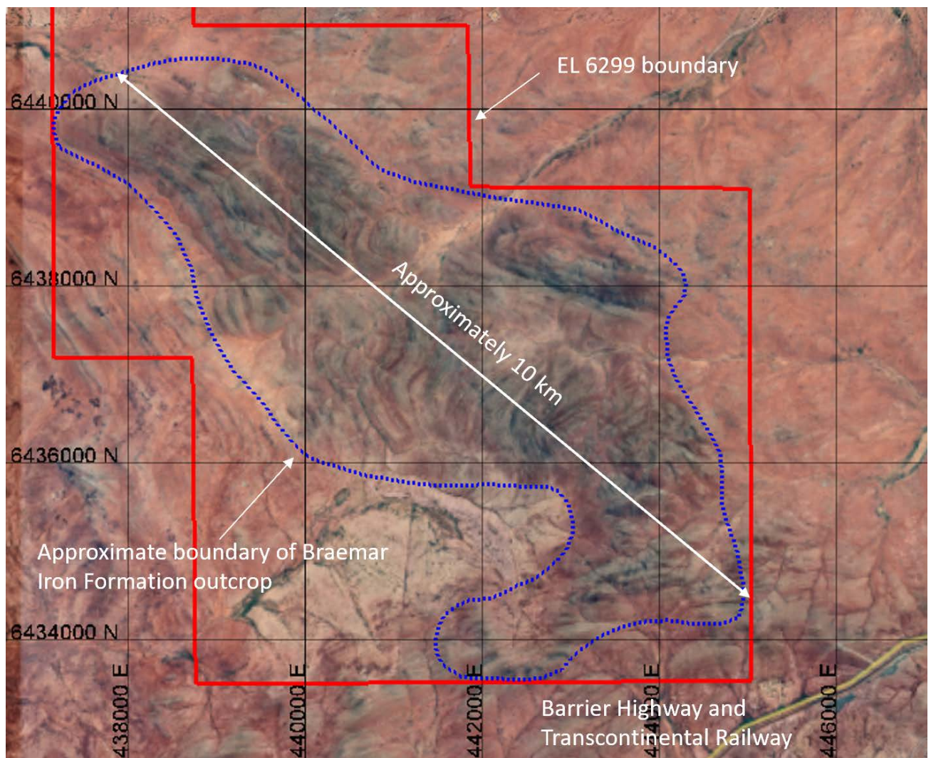
Figure 6 Satellite image showing distinctive dark outcrop of Braemar Iron Formation lying within the boundary of EL6299. Note proximity of Barrier Highway and Transcontinental Railway line to the south.
