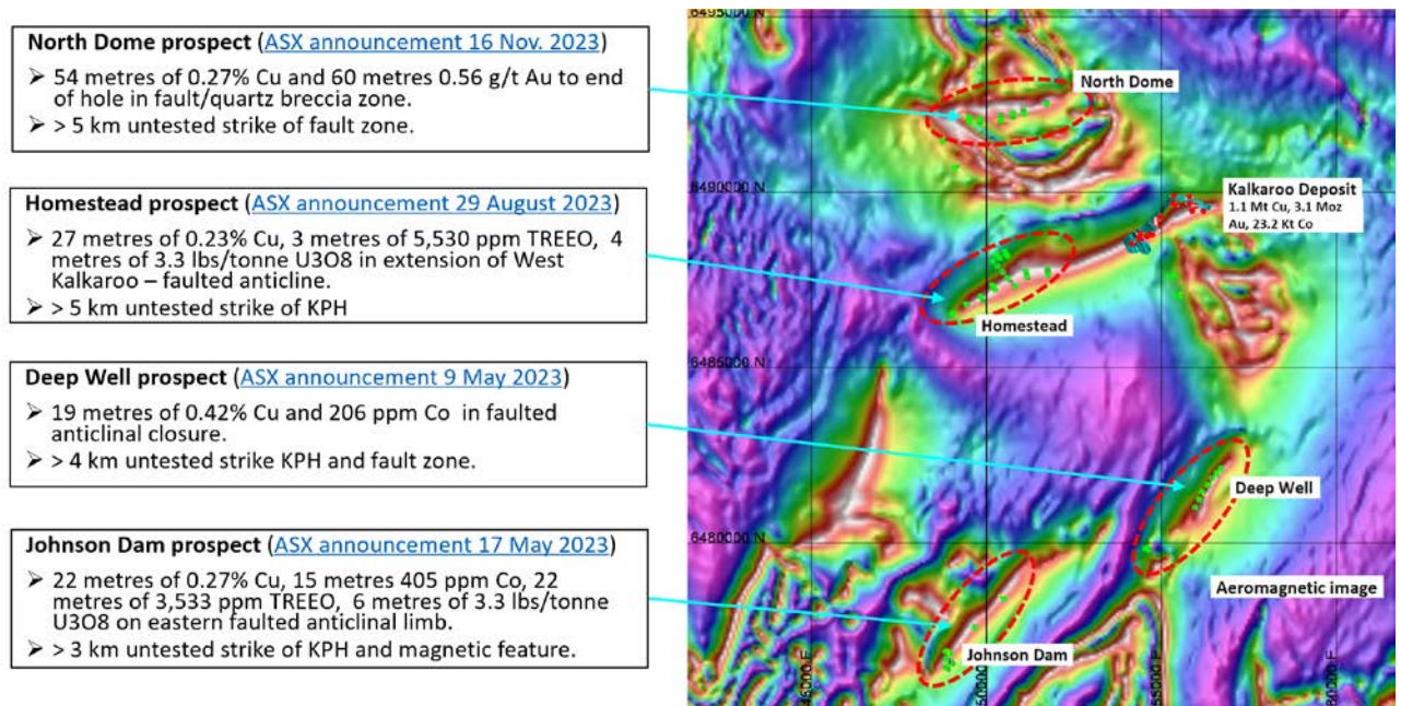
Figure 2 Locations and attribute summaries relating to each of the four key prospects near Kalkaroo plotted on an aeromagnetic image. Note that KPH (Kalkaroo Prospective Horizon) is synonymous with the 'copper horizon' shown in Figure 1.
