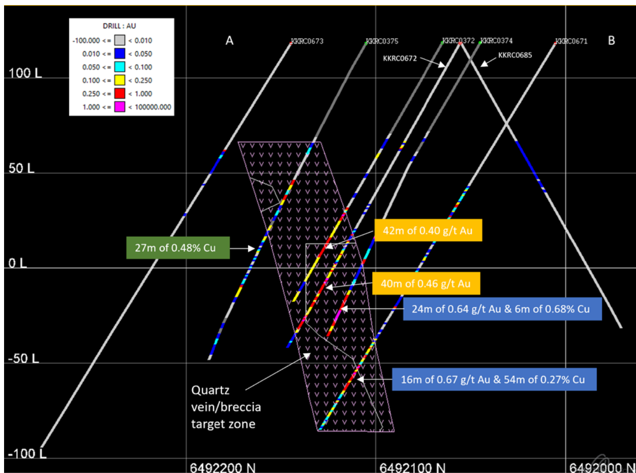
Figure 3 Cross section showing drilling results at the North Dome prospect. The drillholes identify an approximately 40 metre wide zone of well mineralised steeply south-dipping quartz vein/breccia within the fault structure.
