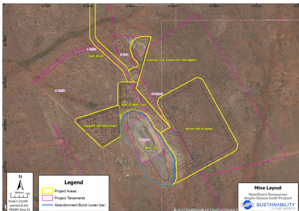
Figure 2. Anglo Saxon Deposit – Proposed Mine Layout
