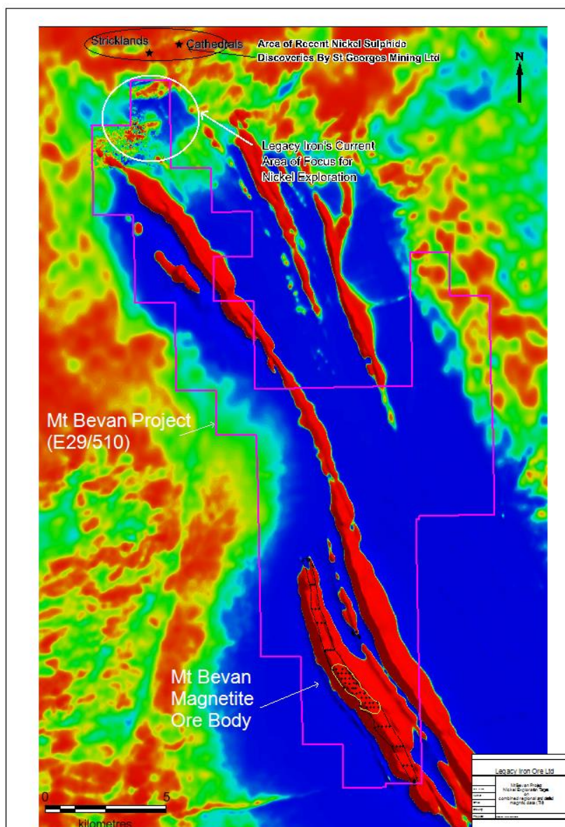
Figure 1 Mt Bevan Project with airborne magnetics (TMI) showing area of interest for nickel sulphide mineralisation
